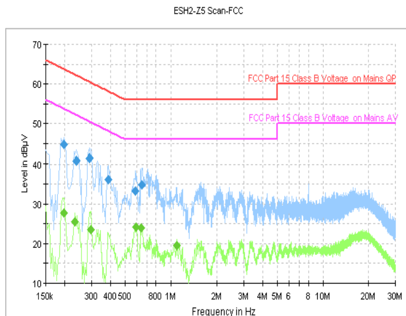
Fig. 18 AC Power line Conducted Emission (Idle, AE3)
