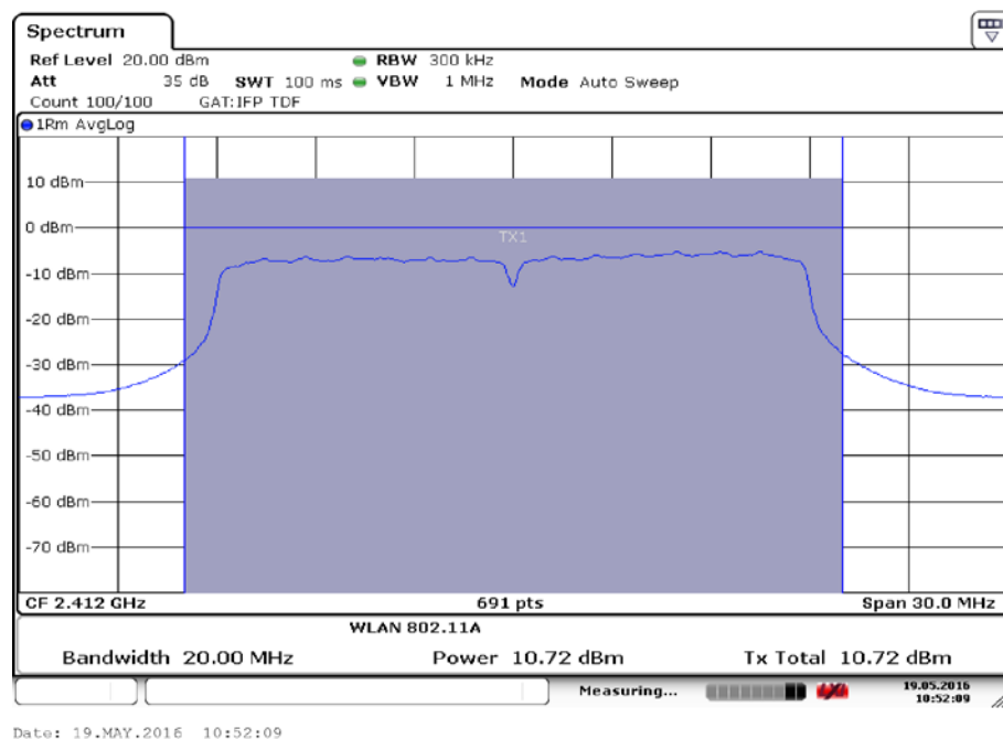
Fig.52 Maximum Average Output Power (802.11n-20MHz, Ch 1,MCS2)
