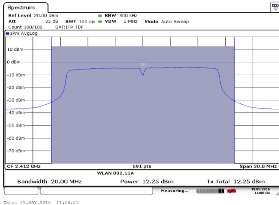
Fig.25 Maximum Average Output Power (802.11g, Ch 1,9Mbps)
