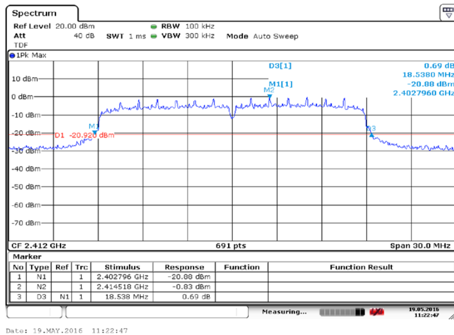
Fig.7 Occupied 20dB Bandwidth (802.11 n-20MHz, Ch 1)
