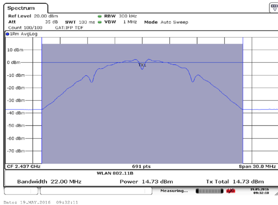
Fig.11 Maximum Average Output Power (802.11b, Ch 6,1Mbps)
