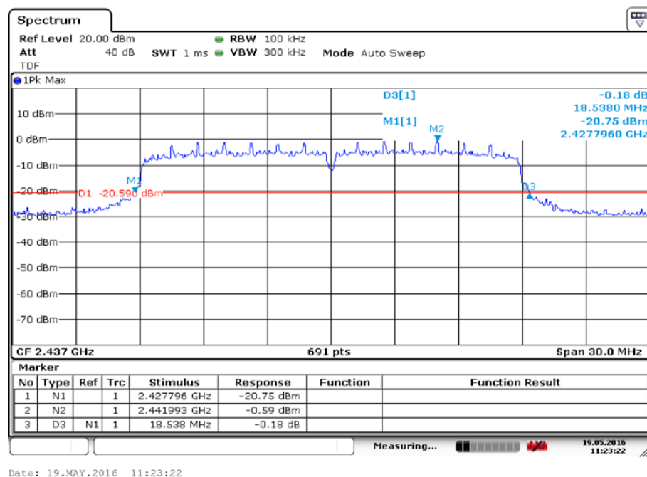
Fig.8 Occupied 20dB Bandwidth (802.11 n-20MHz, Ch 6)
