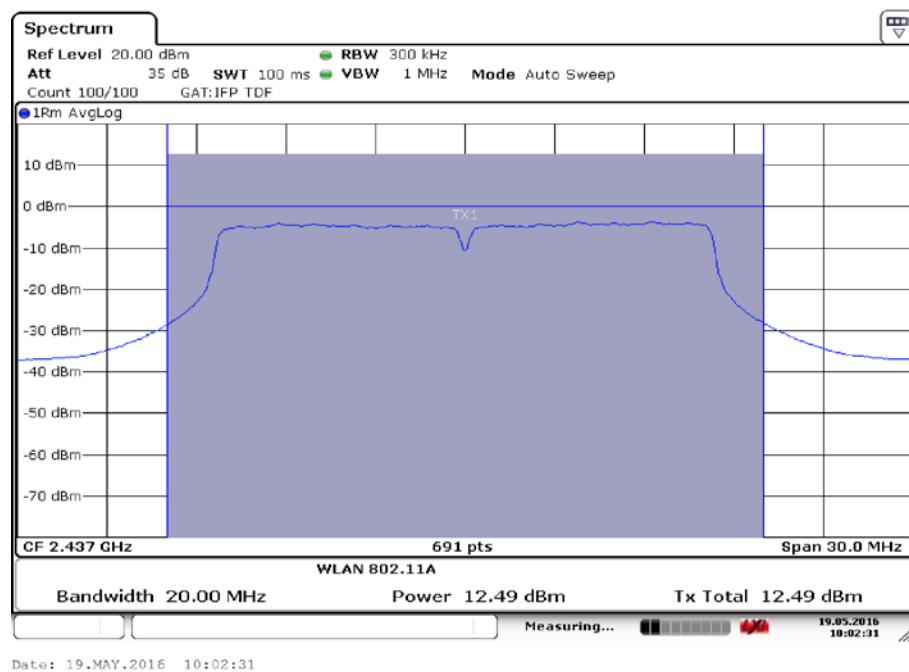
Fig.44 Maximum Average Output Power (802.11g, Ch 6,54Mbps)
