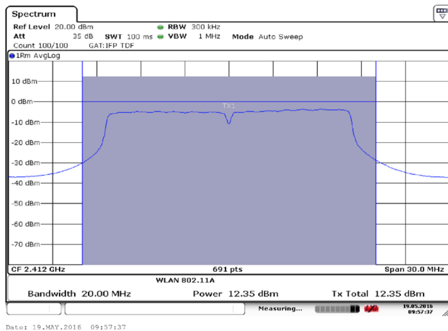
Fig.34 Maximum Average Output Power (802.11g, Ch 1,24Mbps)
