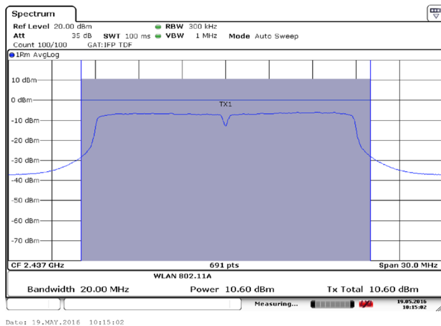
Fig.56 Maximum Average Output Power (802.11n-20MHz, Ch 6,MCS3)
