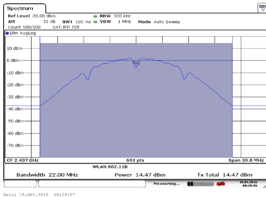
Fig.14 Maximum Average Output Power (802.11b, Ch 6,2Mbps)
