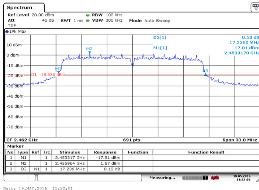
Fig.6 Occupied 20dB Bandwidth (802.11g, Ch 11)
