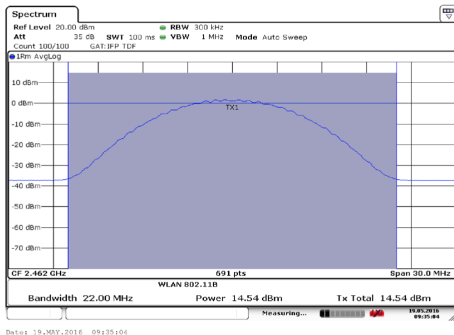
Fig.18 Maximum Average Output Power (802.11b, Ch 11,5.5Mbps)
