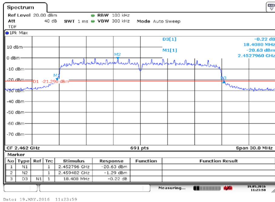
Fig.9 Occupied 20dB Bandwidth (802.11 n-20MHz, Ch 11)
