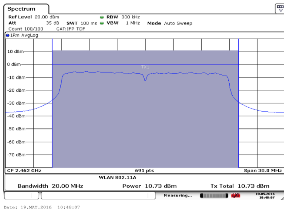
Fig.54 Maximum Average Output Power (802.11n-20MHz, Ch 11,MCS2)
