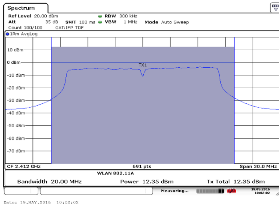
Fig.43 Maximum Average Output Power (802.11g, Ch 1,54Mbps)
