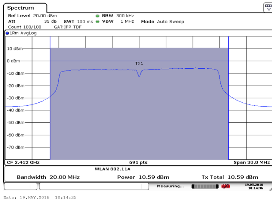
Fig.55 Maximum Average Output Power (802.11n-20MHz, Ch 1,MCS3)
