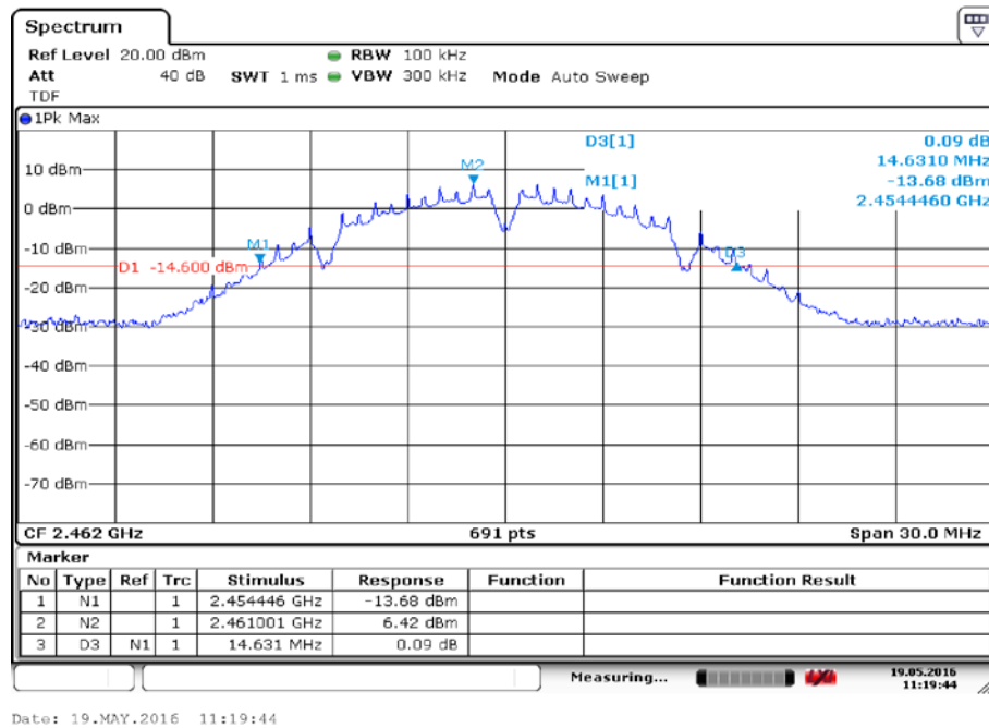
Fig.3 Occupied 20dB Bandwidth (802.11b, Ch 11)
