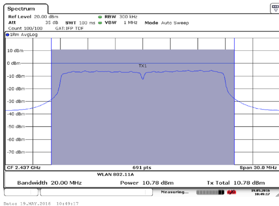
Fig.50 Maximum Average Output Power (802.11n-20MHz, Ch 6,MCS1)
