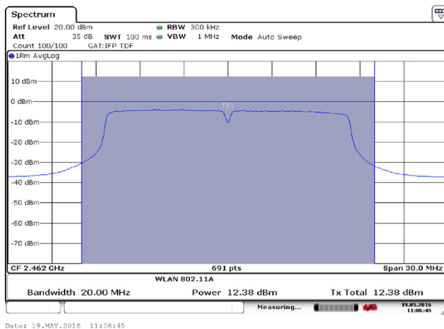
Fig.27 Maximum Average Output Power (802.11g, Ch 11,9Mbps)
