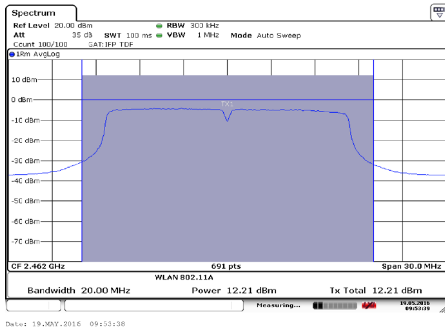
Fig.33 Maximum Average Output Power (802.11g, Ch 11,18Mbps)
