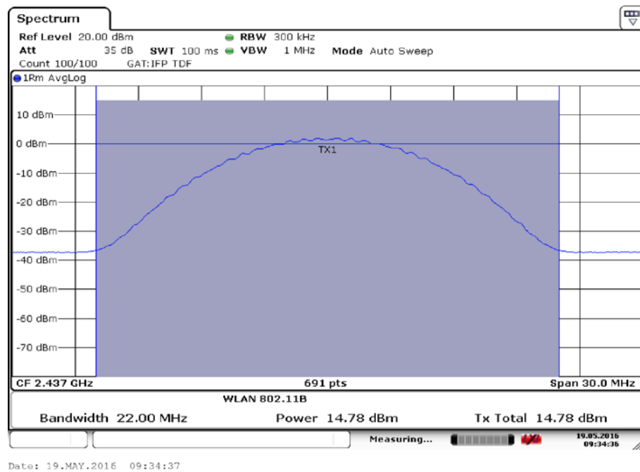
Fig.17 Maximum Average Output Power (802.11b, Ch 6,5.5Mbps)
