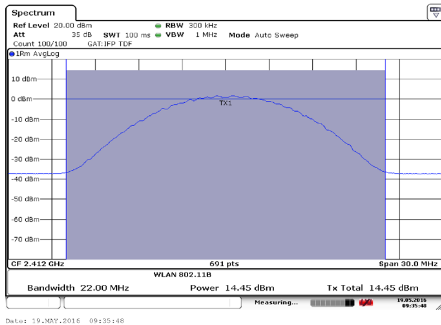
Fig.19 Maximum Average Output Power (802.11b, Ch 1,11Mbps)
