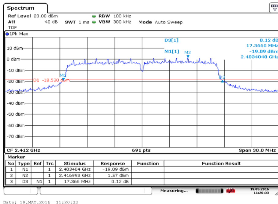
Fig.4 Occupied 20dB Bandwidth (802.11g, Ch 1)
