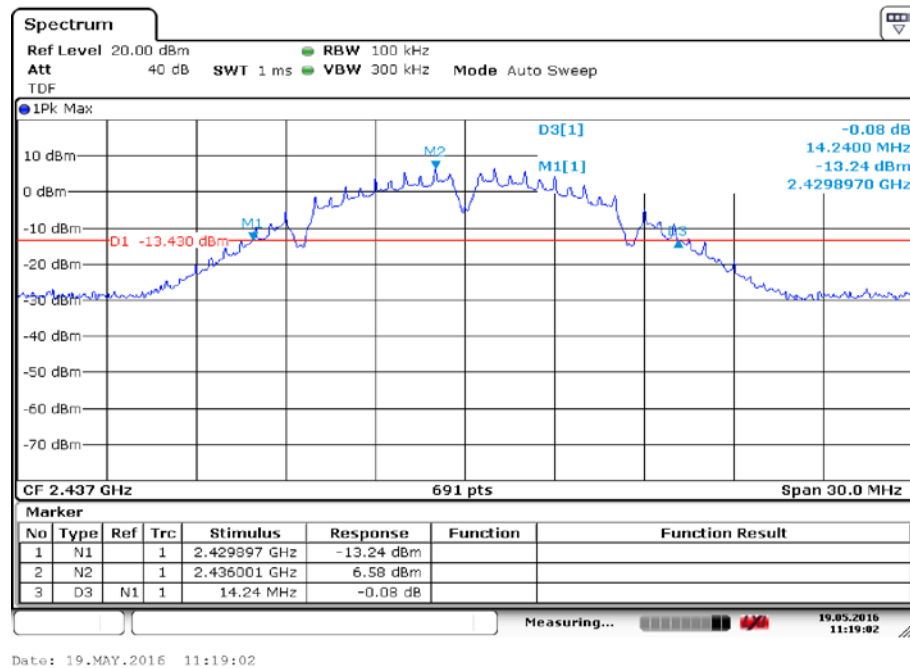
Fig.2 Occupied 20dB Bandwidth (802.11b, Ch 6)
