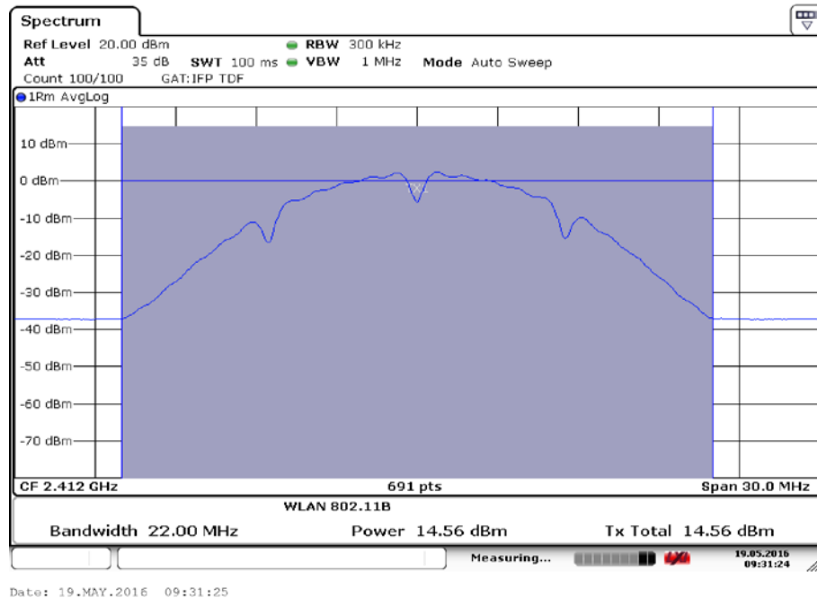
Fig.10 Maximum Average Output Power (802.11b, Ch 1,1Mbps)
