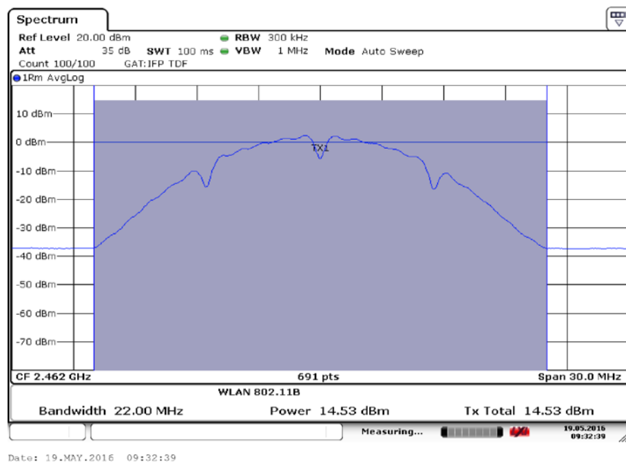
Fig.12 Maximum Average Output Power (802.11b, Ch 11,1Mbps)
