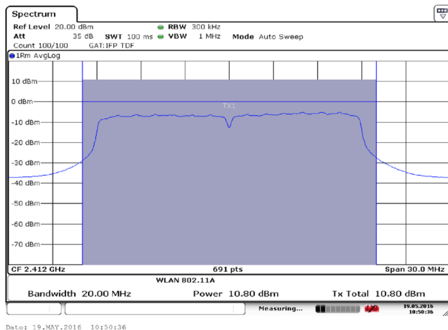
Fig.46 Maximum Average Output Power (802.11n-20MHz, Ch 1,MCS0)
