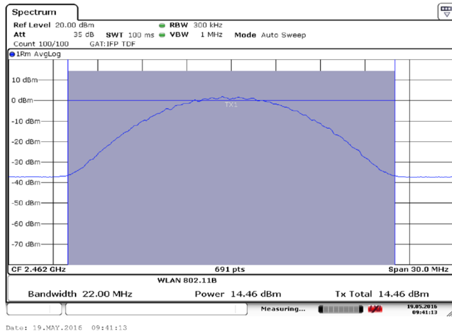
Fig.21 Maximum Average Output Power (802.11b, Ch 11,11Mbps)
