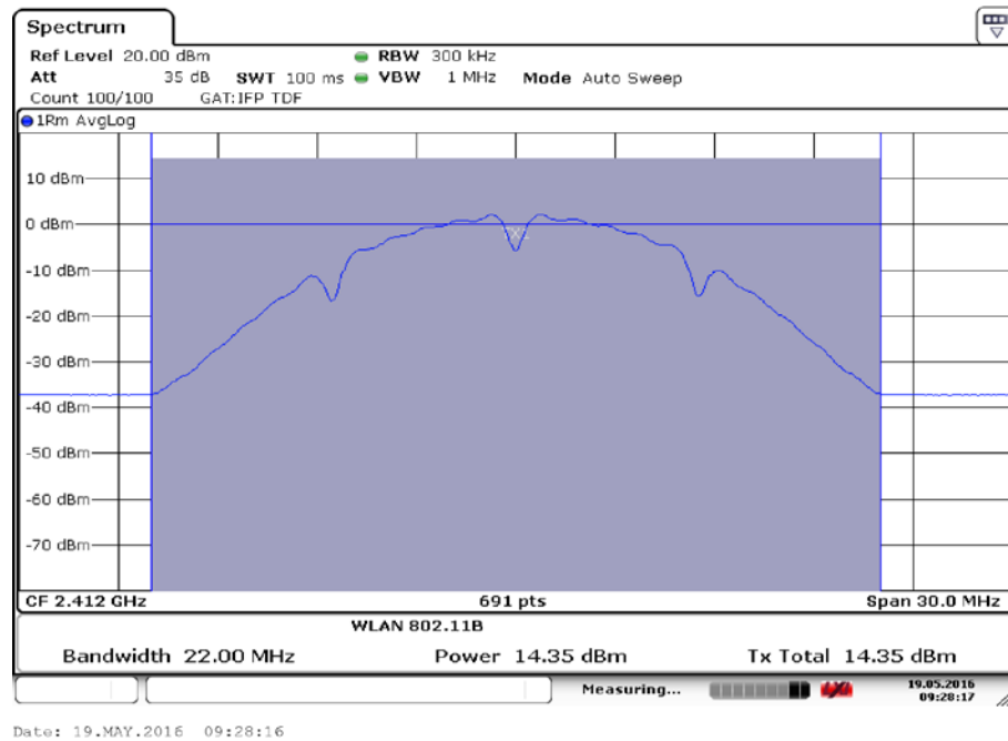
Fig.13 Maximum Average Output Power (802.11b, Ch 1,2Mbps)
