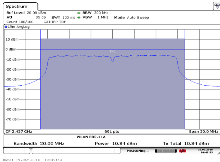
Fig.47 Maximum Average Output Power (802.11n-20MHz, Ch 6,MCS0)
