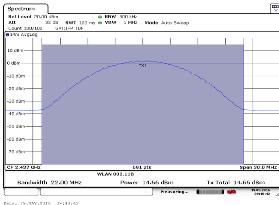
Fig.20 Maximum Average Output Power (802.11b, Ch 6,11Mbps)
