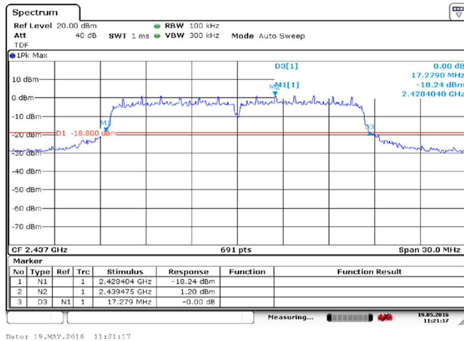
Fig.5 Occupied 20dB Bandwidth (802.11g, Ch 6)
