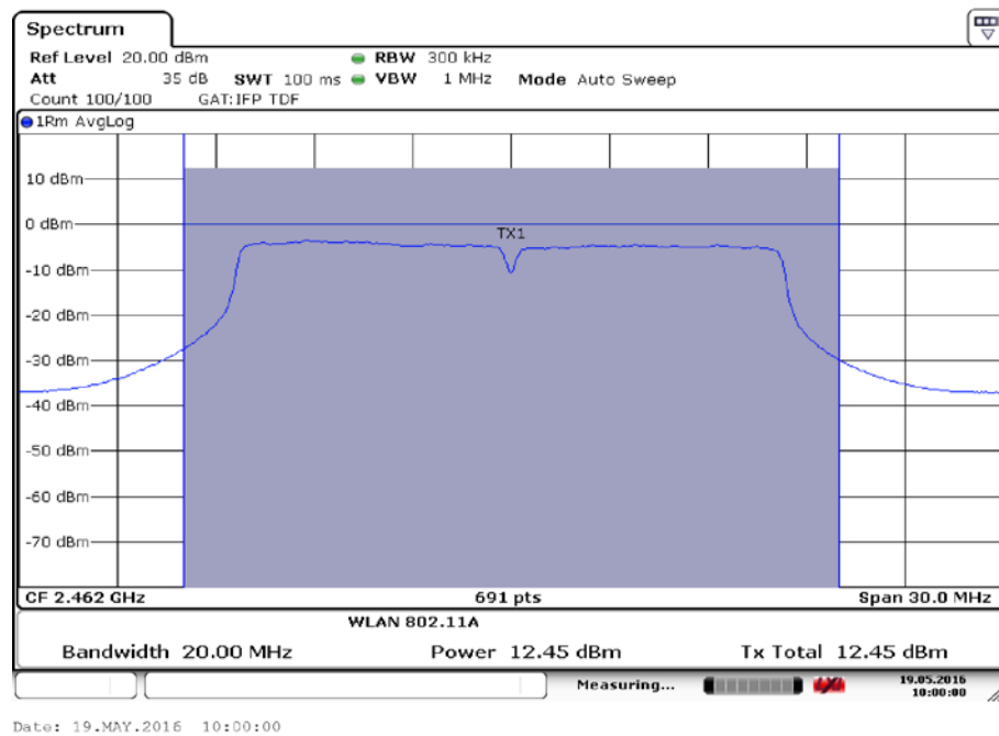
Fig.39 Maximum Average Output Power (802.11g, Ch 11,36Mbps)
