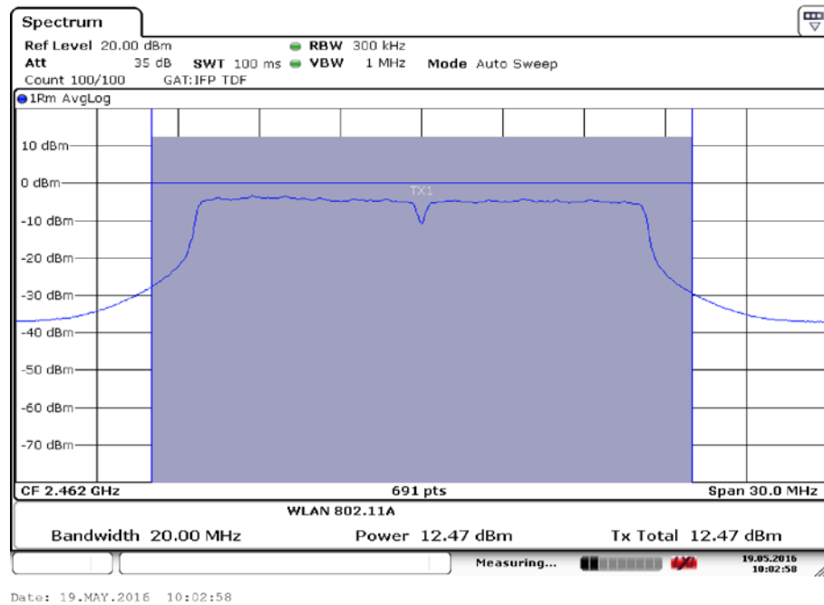
Fig.45 Maximum Average Output Power (802.11g, Ch 11,54Mbps)
