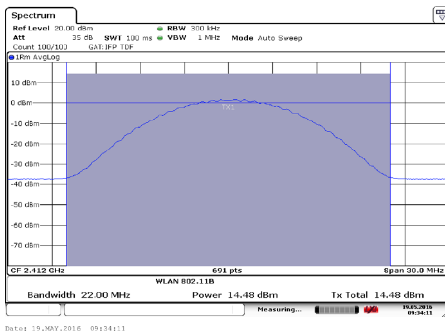
Fig.16 Maximum Average Output Power (802.11b, Ch 1,5.5Mbps)
