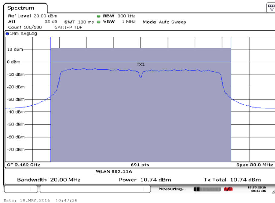
Fig.51 Maximum Average Output Power (802.11n-20MHz, Ch 11,MCS1)
