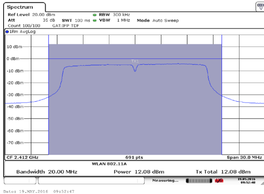
Fig.31 Maximum Average Output Power (802.11g, Ch 1,18Mbps)
