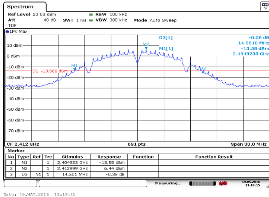
Fig.1 Occupied 20dB Bandwidth (802.11b, Ch 1)
