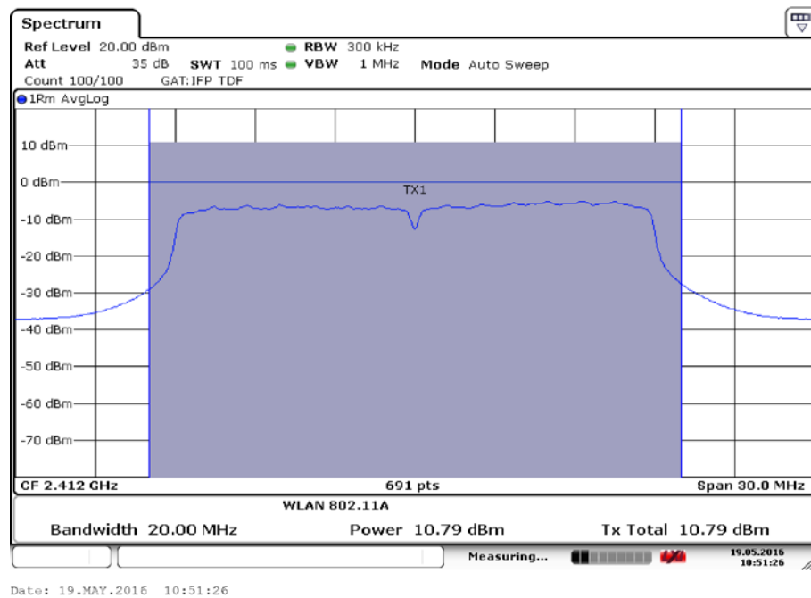
Fig.49 Maximum Average Output Power (802.11n-20MHz, Ch 1,MCS1)
