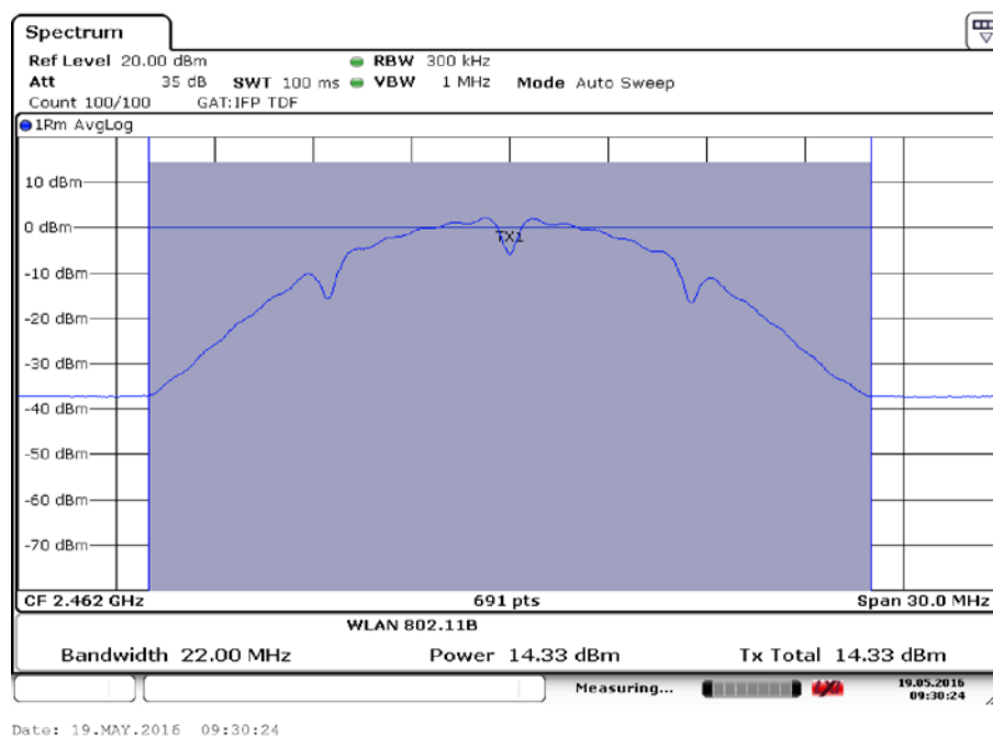
Fig.15 Maximum Average Output Power (802.11b, Ch 11,2Mbps)
