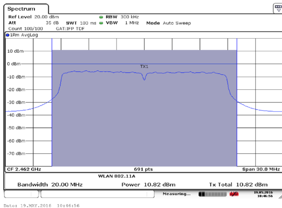
Fig.48 Maximum Average Output Power (802.11n-20MHz, Ch 11,MCS0)
