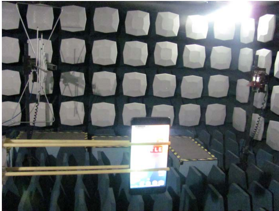
13. Radiated Spurious Emission(Part27)
