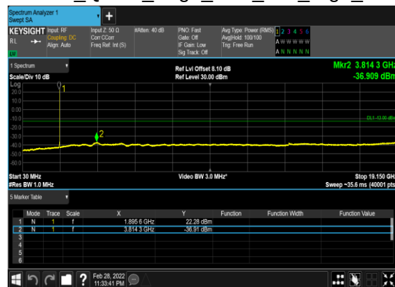
B66_N25(20M)_DFT-s- OFDM_QPSK_Edge_1RB_Left_High_CH
