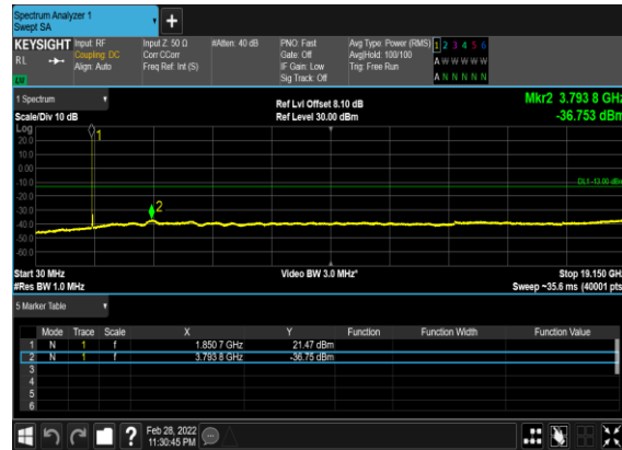
B66_N25(20M)_DFT-s- OFDM_QPSK_Edge_1RB_Left_Low_CH
