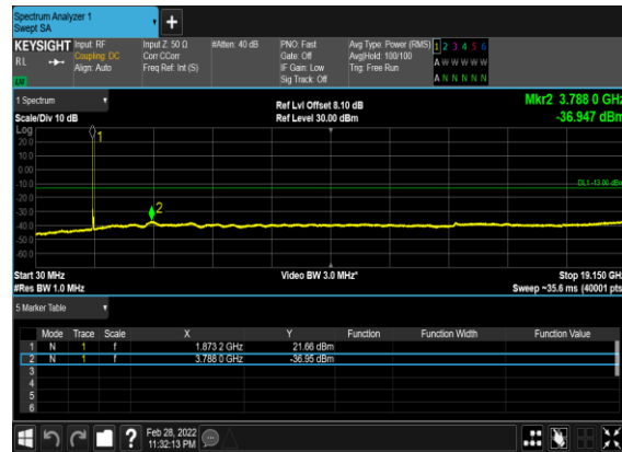
B66_N25(20M)_DFT-s- OFDM_QPSK_Edge_1RB_Left_Mid_CH
