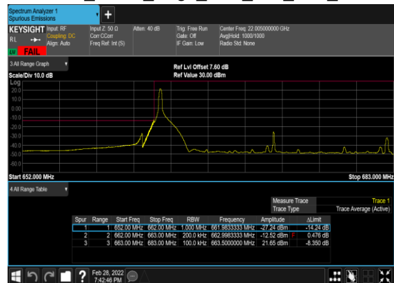
B2_N71(20M)_DFT-s- OFDM_BPSK_Edge_1RB_Left_Low_CH
