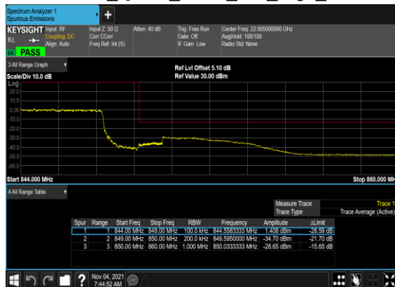
B2_N5(20M)_DFT-s- OFDM_QPSK_Outer_Full_High_CH
