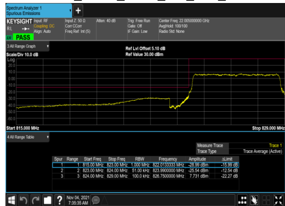
B2_N5(5M)_DFT-s-OFDM_BPSK_Outer_Full_Low_CH
