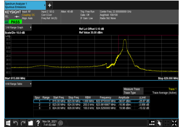
B2_N5(20M)_DFT-s- OFDM_BPSK_Edge_1RB_Left_Low_CH
