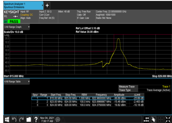
B2_N5(10M)_DFT-s- OFDM_BPSK_Edge_1RB_Left_Low_CH
