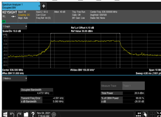
B2_N5(5M)_CP-OFDM_64 QAM_Outer_Full_Mid_CH
