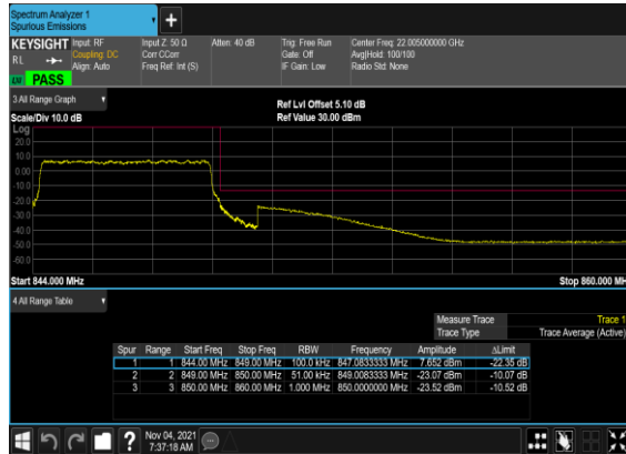
B2_N5(5M)_DFT-s- OFDM_QPSK_Outer_Full_High_CH
