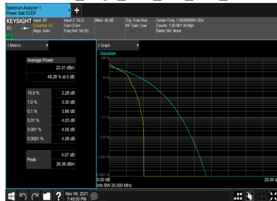
B12_N25(20M)_DFT-s-OFDM_PI_2-BPSK_Edge_1RB_Left_Low_CH
