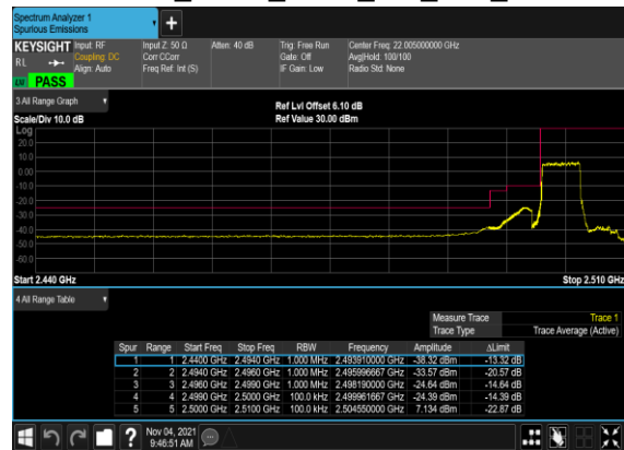
B5_N7(5M)_DFT-s-OFDM_BPSK_Outer_Full_Low_CH
