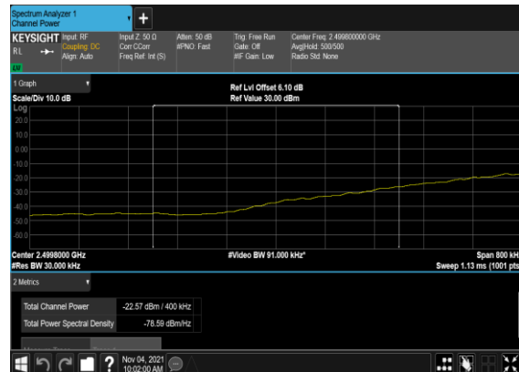
B5_N7(20M)_DFT-s- OFDM_BPSK_Edge_1RB_Left_Low_CH_chP_PASS
