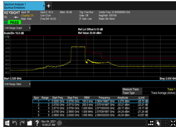
B5_N7(10M)_DFT-s- OFDM_QPSK_Outer_Full_High_CH
