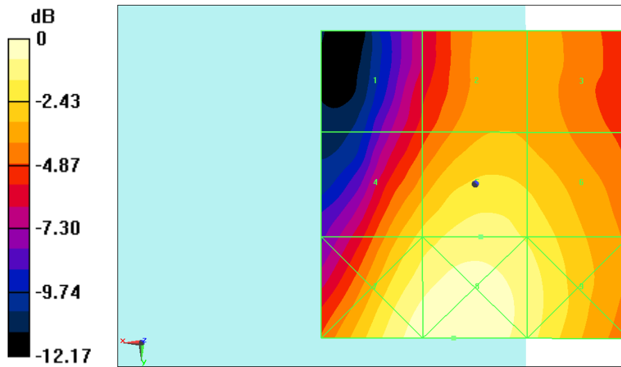
Fig B.4 HAC RF E-Field LTE Band38 QPSK CH38750
