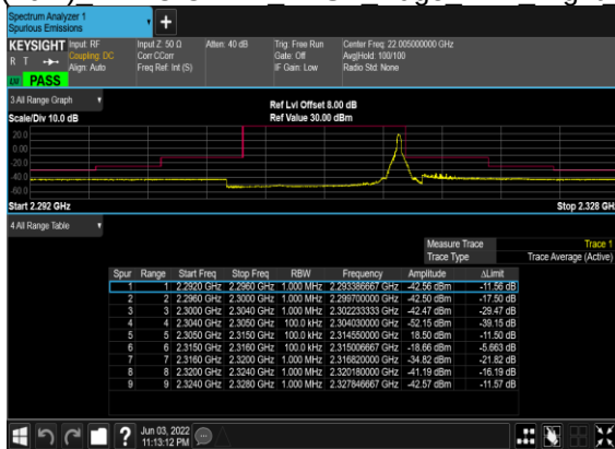
B5_N30(10M) DFT-s-OFDM BPSK Edge 1RB Right Low_CH
