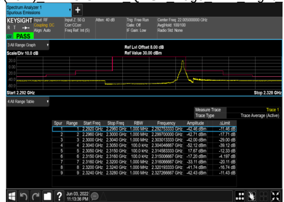
B5_N30(10M) DFT-s-OFDM QPSK Edge 1RB Right Low_CH
