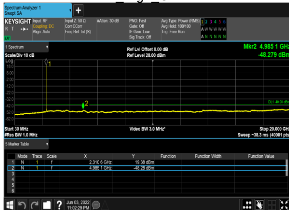
B5_N30(5M)_DFT-s-OFDM_QPSK_Edge_1RB_Left High_CH
