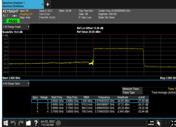
B5_N77(60M)_DFT-s- OFDM_QPSK_Outer_Full_Low_CH
