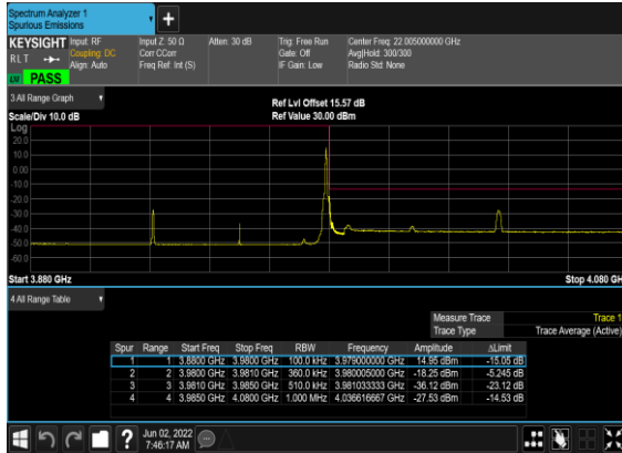
B5_N77(60M)_DFT-s- OFDM_QPSK_Edge_1RB_Right_High_CH
