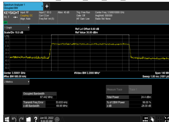
B5_N77(70M)_CP-OFDM_256 QAM_Outer_Full_Mid_CH
