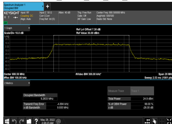
N71(10M)_CP-OFDM_256 QAM_Outer_Full_Mid_CH
