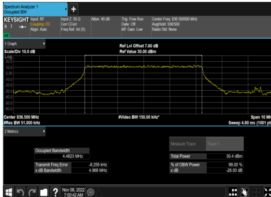
N5(5M)_DFT-s-OFDM_PI_2- BPSK_Outer_Full_Mid_CH
