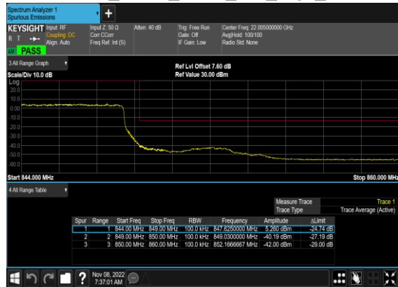
N5(10M)_DFT-s- OFDM_BPSK_Outer_Full_High_CH
