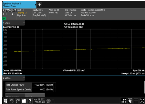
N5(10M)_DFT-s- OFDM_QPSK_Edge_1RB_Left_Low_CH_CHP_PASS
