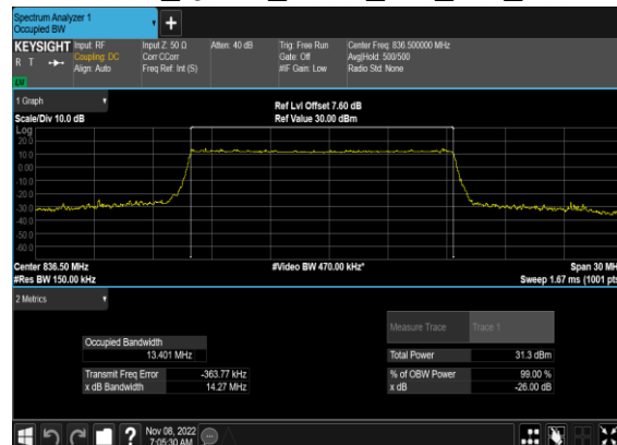
N5(15M)_DFT-s- OFDM_QPSK_Outer_Full_Mid_CH
