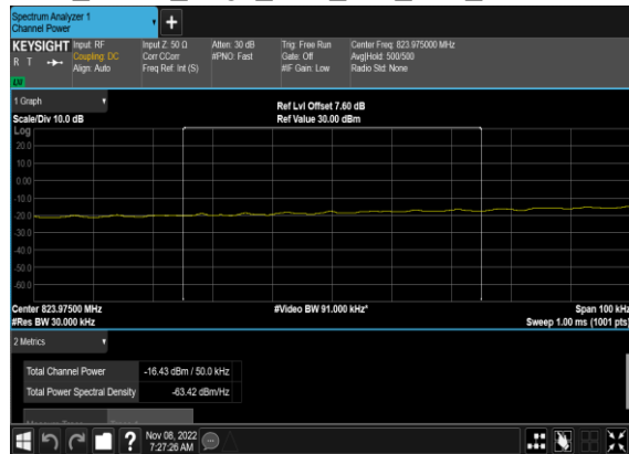
N5(5M)_DFT-s- OFDM_QPSK_Edge_1RB_Left_Low_CH_chp_PASS
