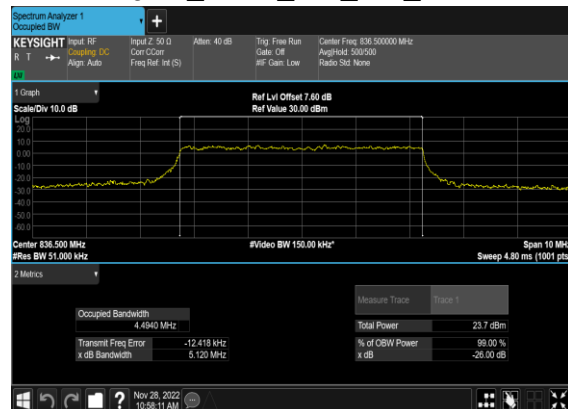
N5(5M)_CP-OFDM_256 QAM_Outer_Full_Mid_CH
