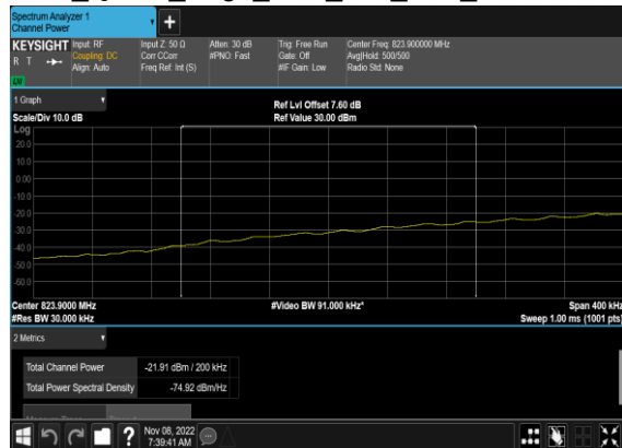
N5(20M)_DFT-s- OFDM_QPSK_Edge_1RB_Left_Low_CH_CHP_PASS
