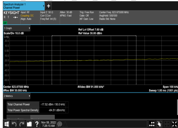
N5(5M)_DFT-s- OFDM_BPSK_Edge_1RB_Left_Low_CH_chp_PASS
