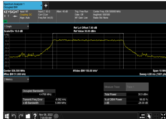
N5(5M)_DFT-s- OFDM_QPSK_Outer_Full_Mid_CH
