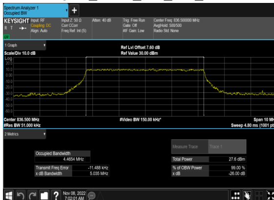
N5(5M)_CP-OFDM_64 QAM_Outer_Full_Mid_CH
