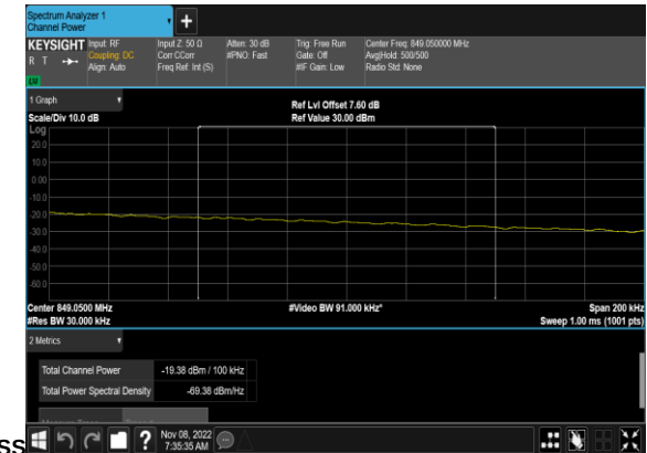
N5(10M)_DFT-s- OFDM_BPSK_Edge_1RB_Right_High_CH_CHP_PA
