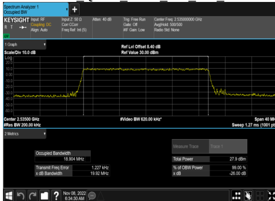
N7(20M)_CP- OFDM QPSK Outer Full Mid CH
