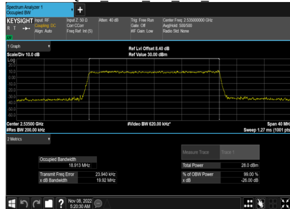
N7(20M)_CP-OFDM_16 QAM Outer Full Mid CH
