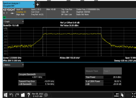
N7(5M)_CP-OFDM_16 QAM Outer Full Mid CH
