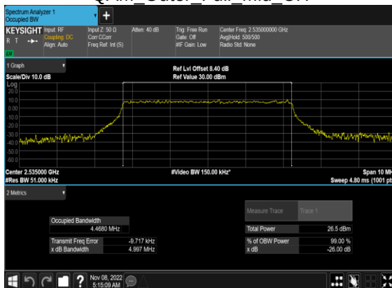
N7(5M)_CP-OFDM_64 QAM Outer Full Mid CH
