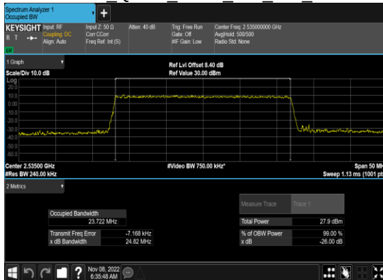
N7(25M)_CP- OFDM QPSK Outer Full Mid CH
