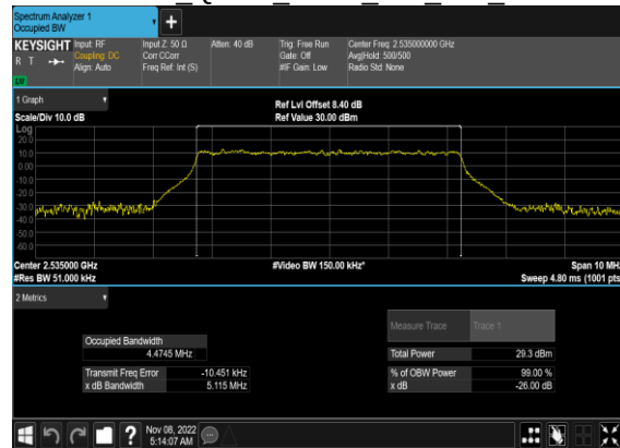
N7(5M)_DFT-s- OFDM QPSK Outer Full Mid CH
