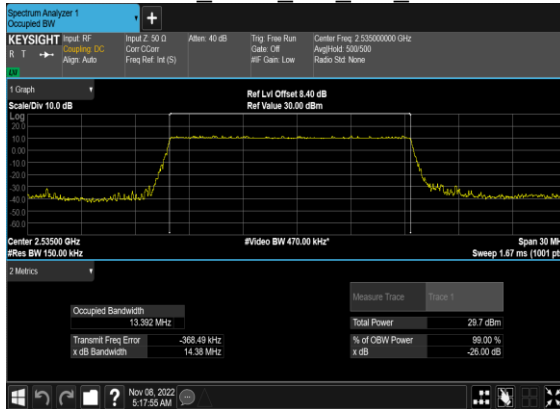
N7(15M)_DFT-s-OFDM_PI_2- BPSK Outer Full Mid CH
