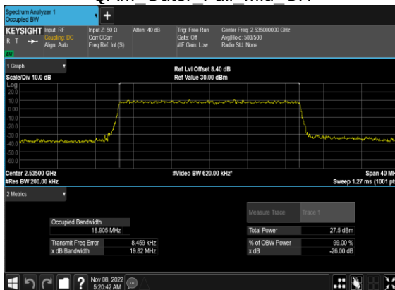
N7(20M)_CP-OFDM_64 QAM Outer Full Mid CH
