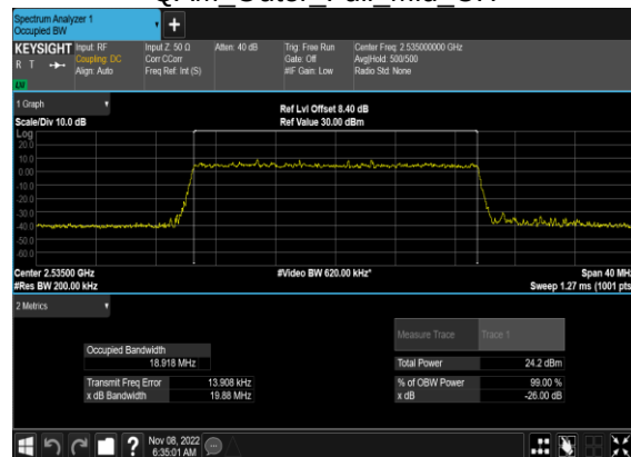
N7(20M)_CP-OFDM_256 QAM Outer Full Mid CH
