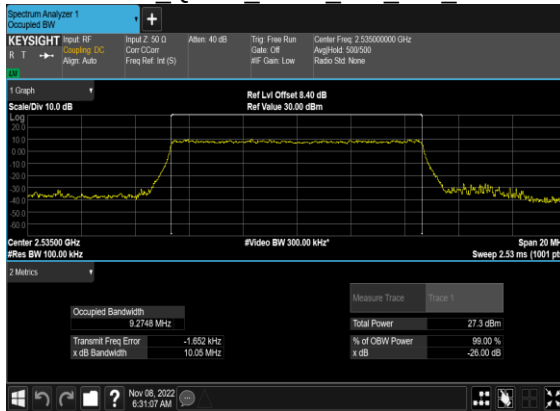
N7(10M)_CP- OFDM QPSK Outer Full Mid CH
