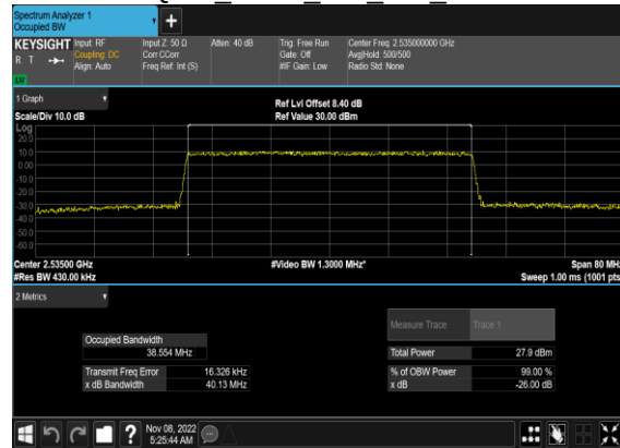
N7(40M)_CP-OFDM_16 QAM Outer Full Mid CH
