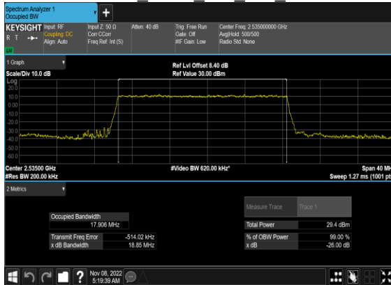
N7(20M)_DFT-s-OFDM_PI_2- BPSK Outer Full Mid CH
