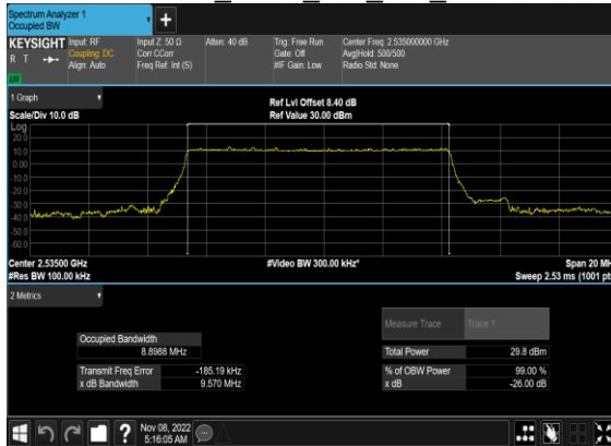
N7(10M)_DFT-s-OFDM_PI_2- BPSK Outer Full Mid CH
