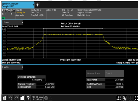
N7(5M)_DFT-s-OFDM_PI_2- BPSK Outer Full Mid CH
