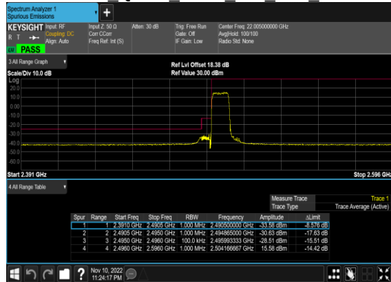
N41(10M)_CP- OFDM QPSK Outer Full Low CH
