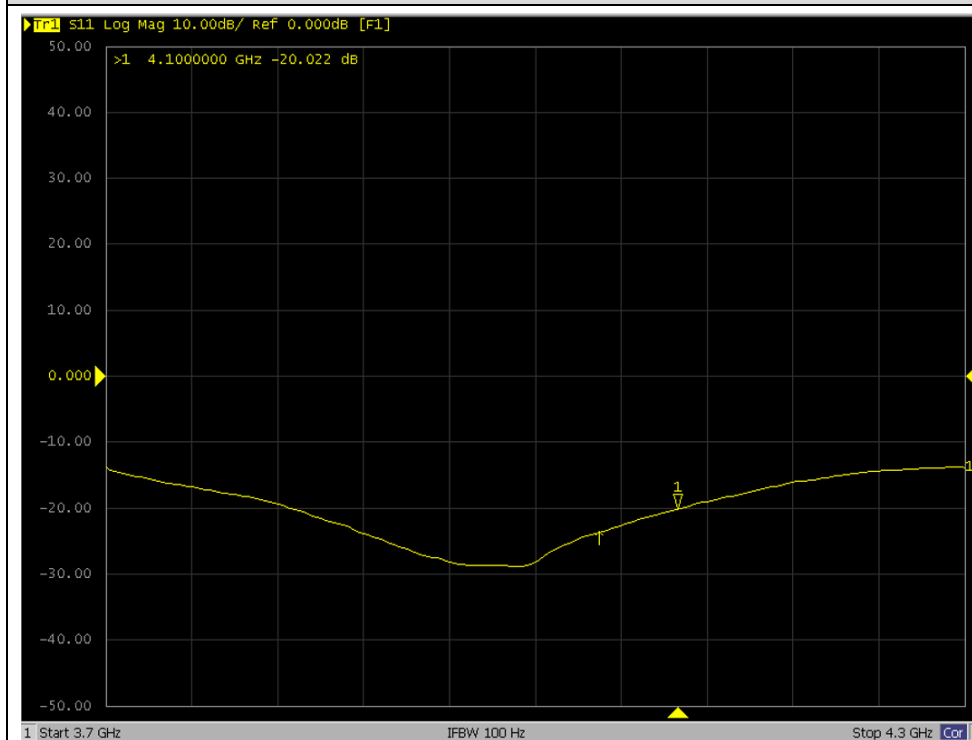
Impedance
