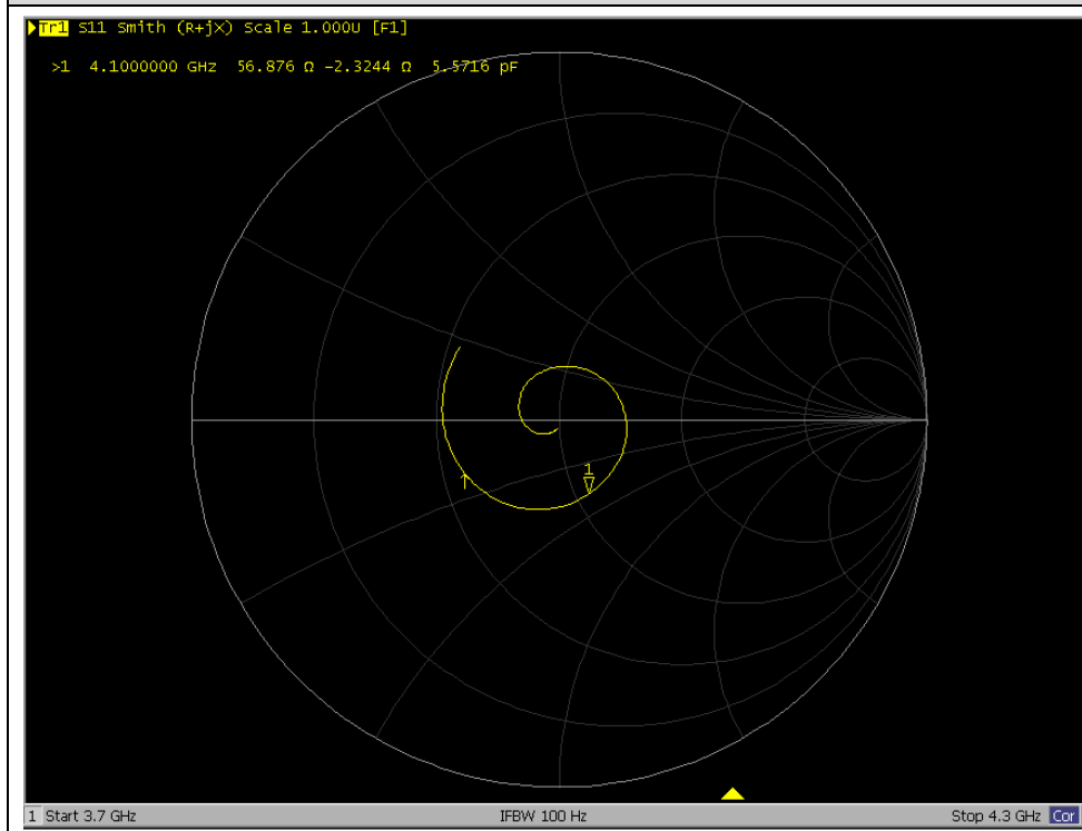
Impedance
