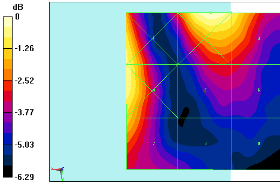
Fig B.1 HAC RF E-Field LTE Band48 QPSK
