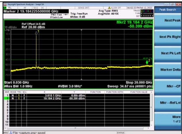
Band48C-30M-20G / 5MHz+20MHz / 25RB+100RB / QPSK / Mid CH
