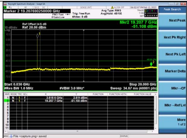
Band48C-30M-20G / 5MHz+20MHz / 1RB+1RB / QPSK / Mid CH
