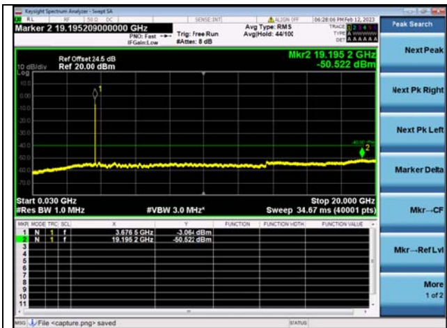
Band48C-30M-20G / 20MHz+5MHz / 1RB+1RB / QPSK / High CH
