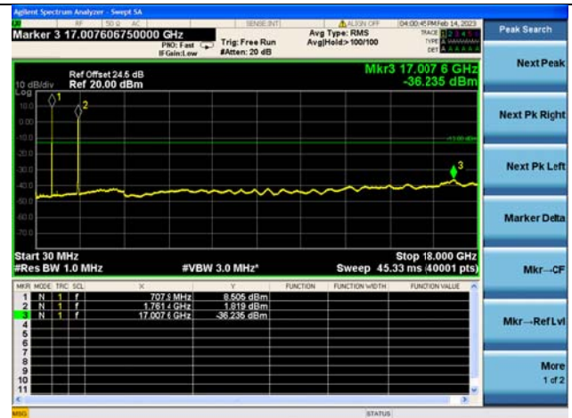
FULLRB QPSK M
