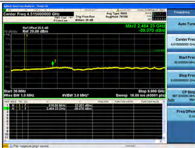
Band26Part90 / 5MHz / High CH / 16QAM
