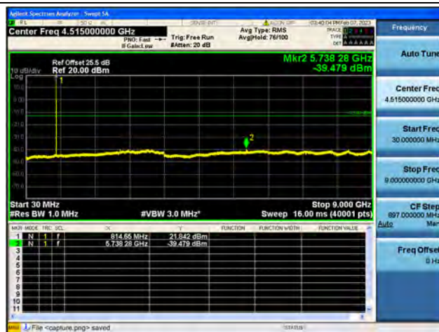
Band26Part90 / 5MHz / Low CH / 16QAM
