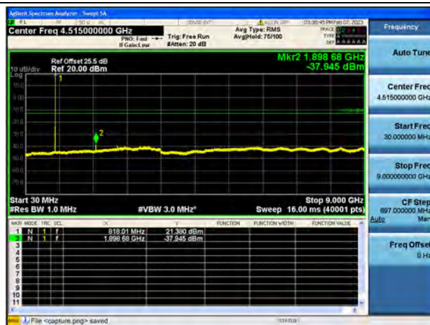
Band26Part90 / 3MHz / Mid CH / 16QAM
