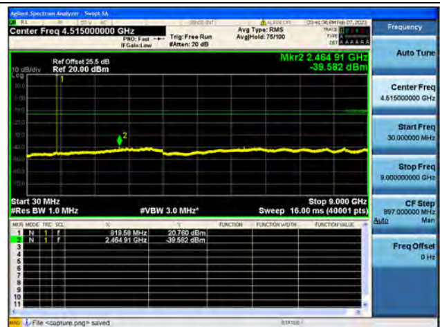
Band26Part90 / 5MHz / High CH / 64QAM
