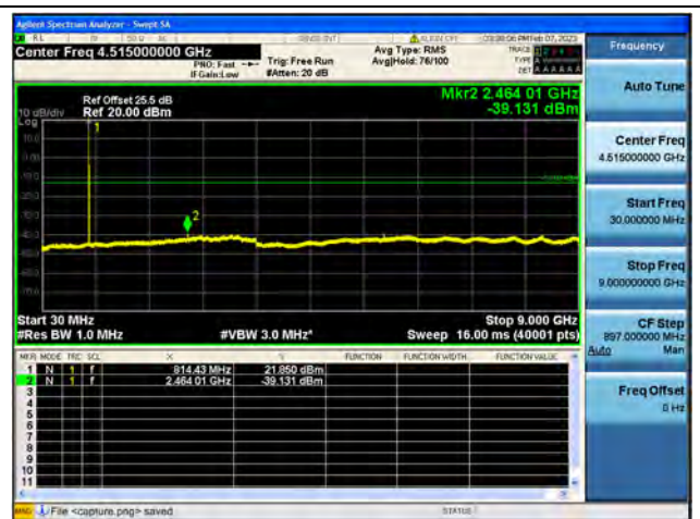
Band26Part90 / 3MHz / Low CH / 16QAM
