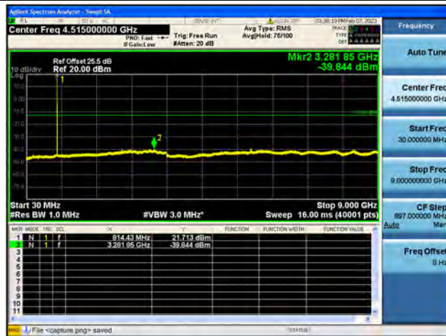
Band26Part90 / 3MHz / Low CH / 64QAM
