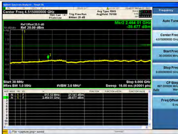
Band26Part90 / 5MHz / Mid CH / 64QAM
