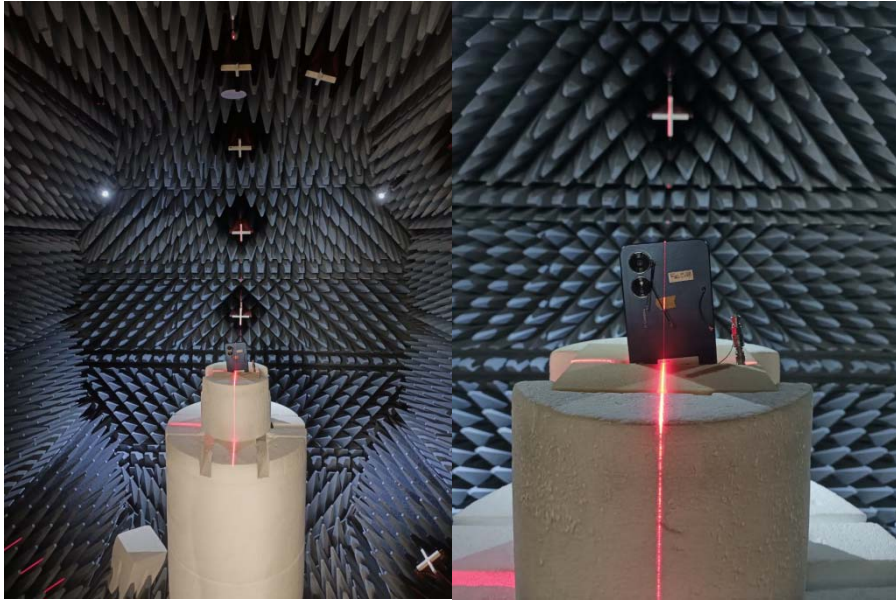
Fig.4. The DUT in the fully anechoic chamber
