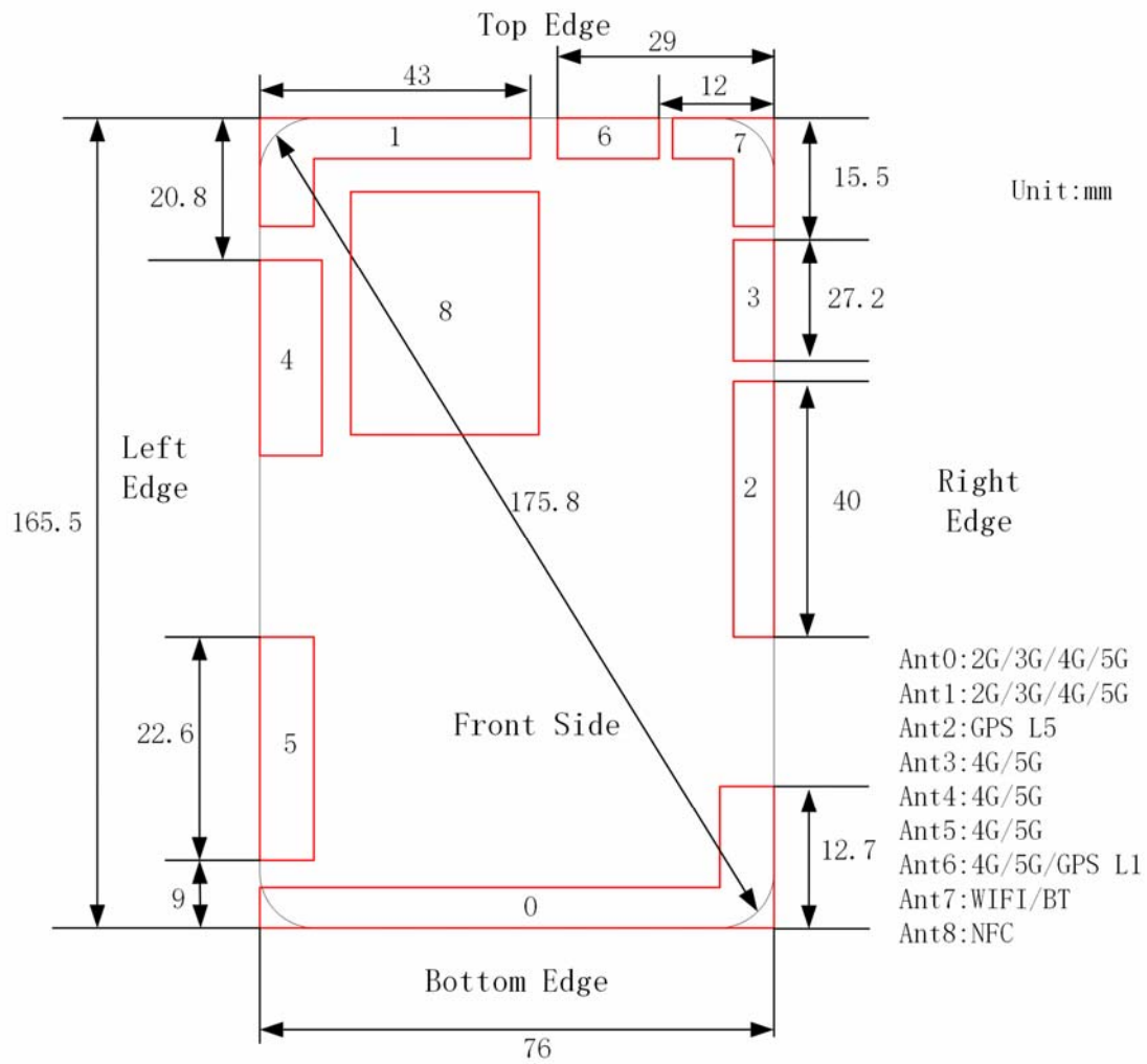
Fig 5 Antenna location&amp;dimension
