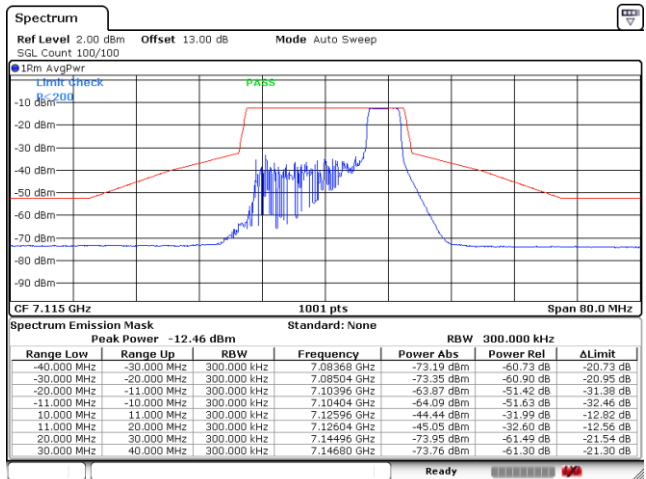
Plot on Channel 7115MHz 52RU40
