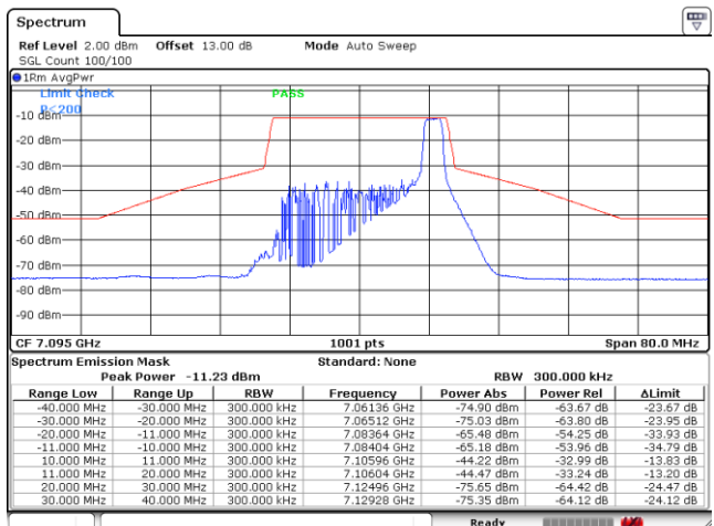
Plot on Channel 7095MHz 26RU8
