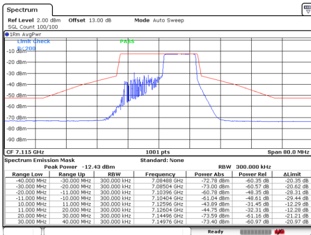
Plot on Channel 7115MHz 106RU54
