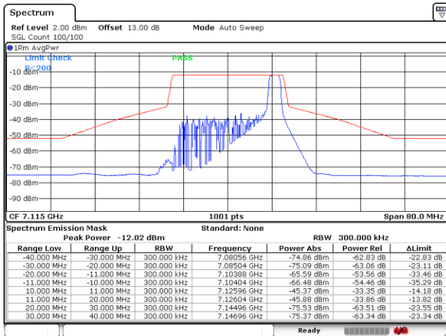
Plot on Channel 7115MHz 26RU8
