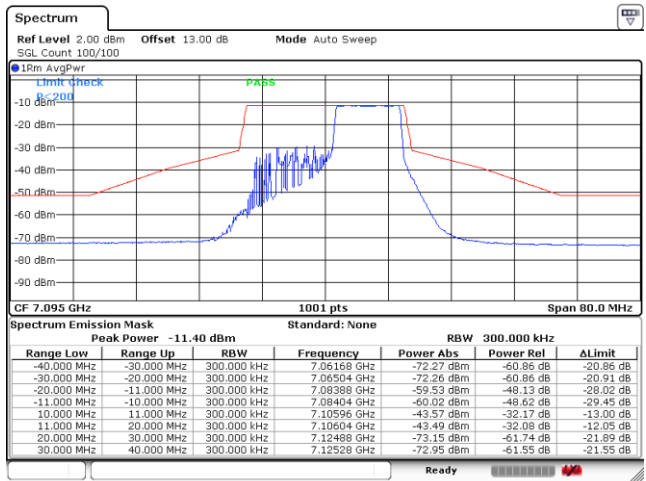
Plot on Channel 7095MHz 106RU54
