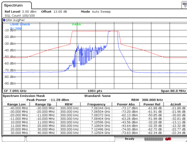
Plot on Channel 7095MHz 52RU40
