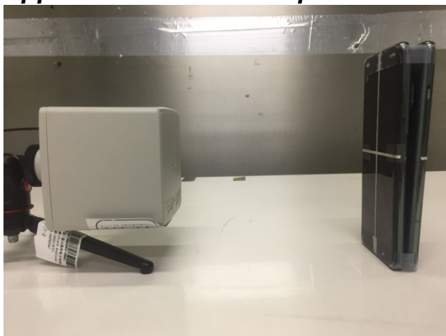
Position A, test separation 20cm
