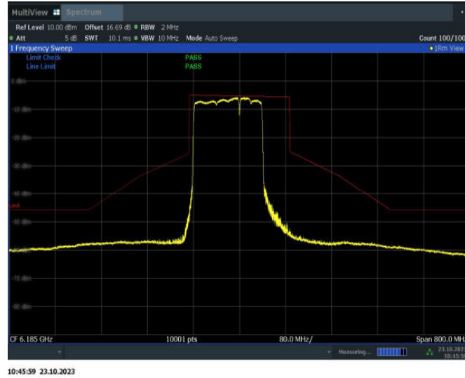
11BE160MIMO_Ant15_6185_996+484+242_OFDMA_1
