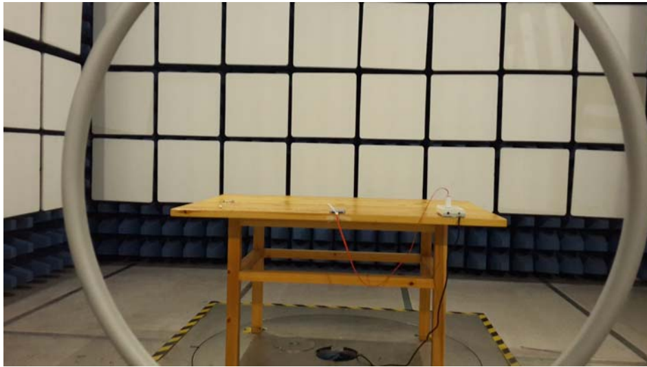
Below 30MHz
