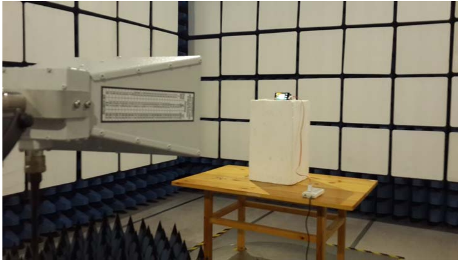
Above 1GHz
