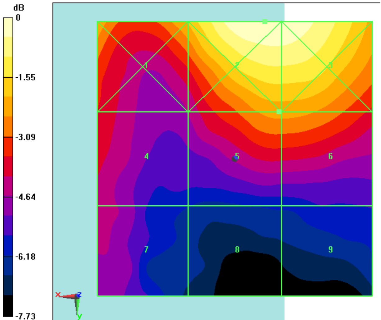
Fig B.48 HAC RF E-Field LTE Band41 Power Class 3 16QAM CH40185
