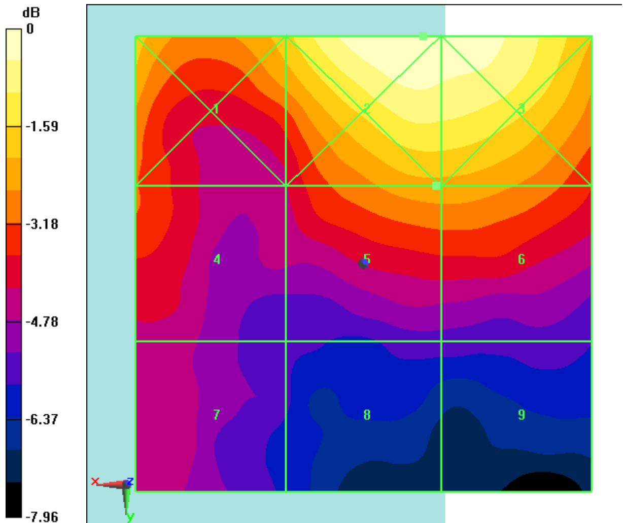
Fig B.38 HAC RF E-Field LTE Band41 Power Class 2 64QAM CH40185
