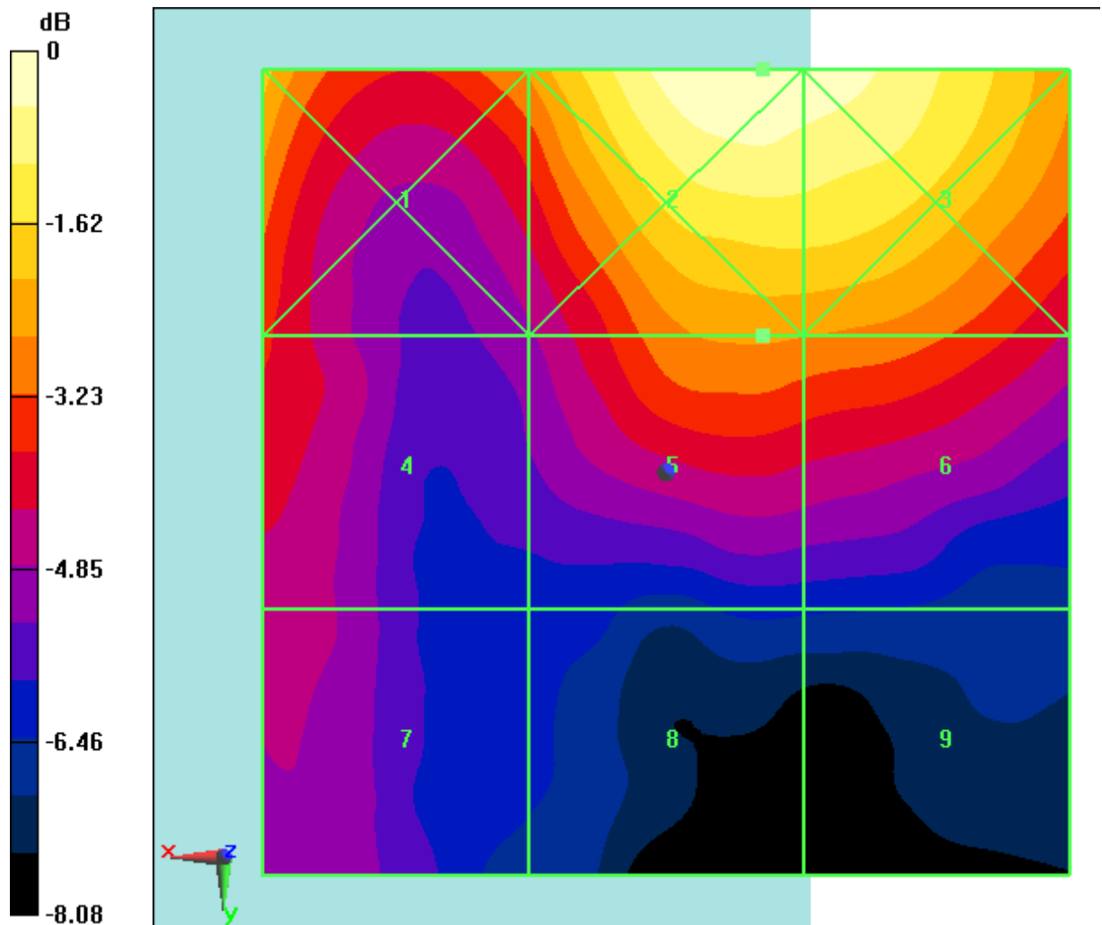
Fig B.36 HAC RF E-Field LTE Band41 Power Class 2 64QAM CH41055
