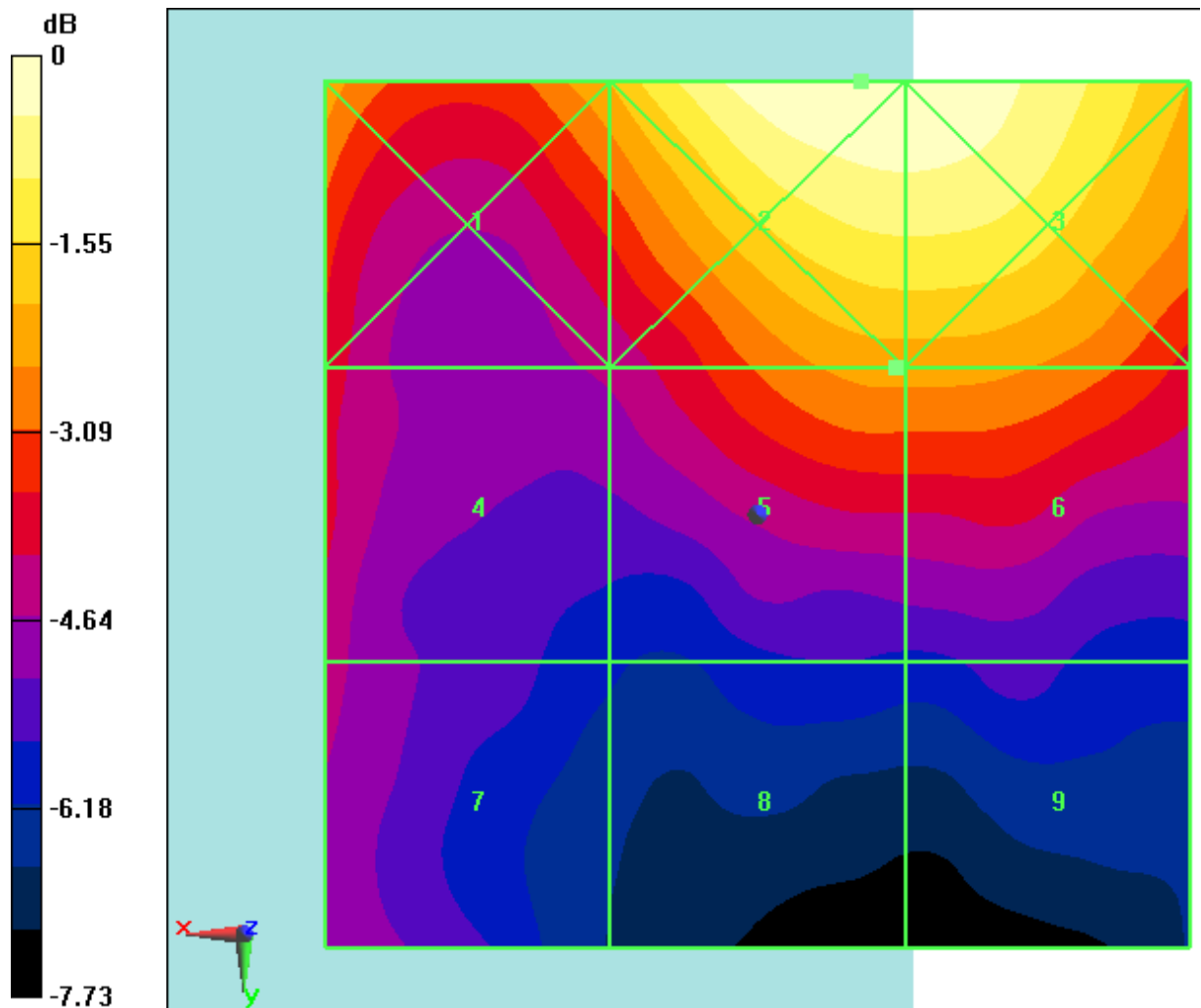
Fig B.28 HAC RF E-Field LTE Band41 Power Class 2 QPSK CH40185
