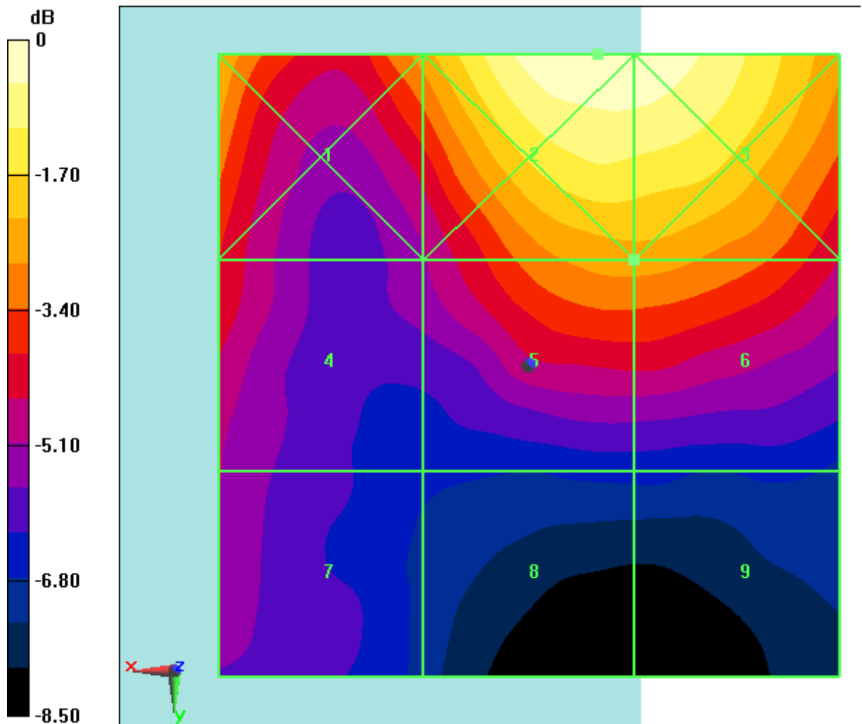
Fig B.41 HAC RF E-Field LTE Band41 Power Class 3 QPSK CH41055
