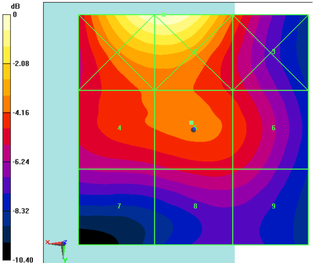
Fig B.23 HAC RF E-Field LTE Band48 64QAM CH55990
