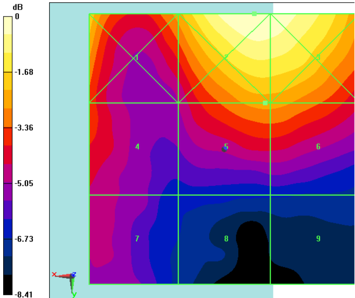
Fig B.31 HAC RF E-Field LTE Band41 Power Class 2 16QAM CH41055
