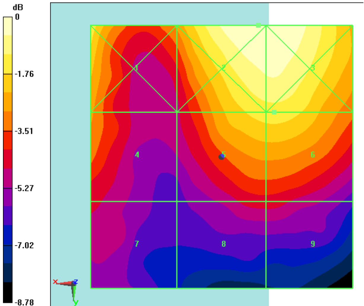
Fig B.30 HAC RF E-Field LTE Band41 Power Class 2 16QAM CH41490
