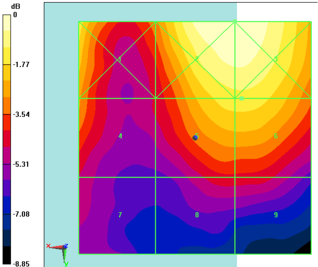
Fig B.25 HAC RF E-Field LTE Band41 Power Class 2 QPSK CH41490
