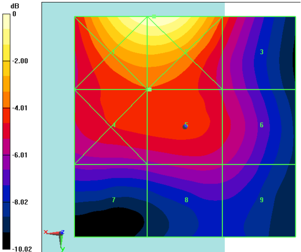
Fig B.22 HAC RF E-Field LTE Band48 64QAM CH56640
