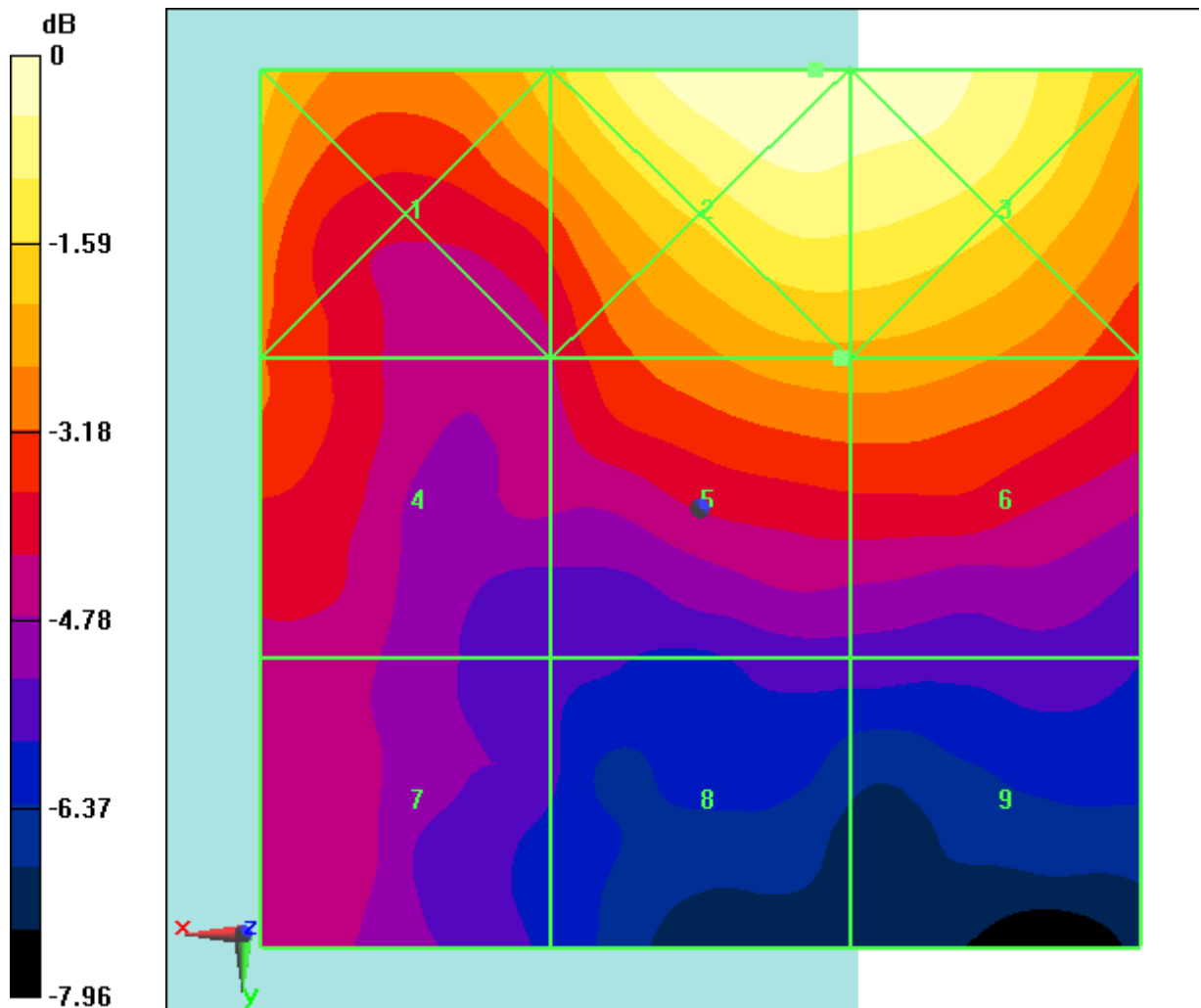
Fig B.53 HAC RF E-Field LTE Band41 Power Class 3 64QAM CH40185
