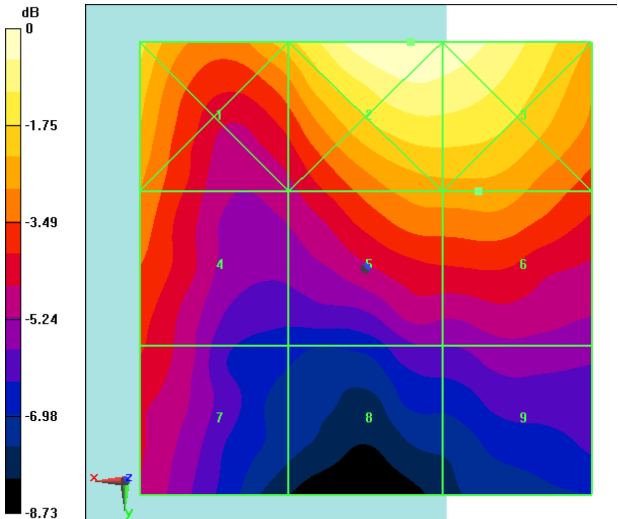
Fig B.47 HAC RF E-Field LTE Band41 Power Class 3 16QAM CH40620
