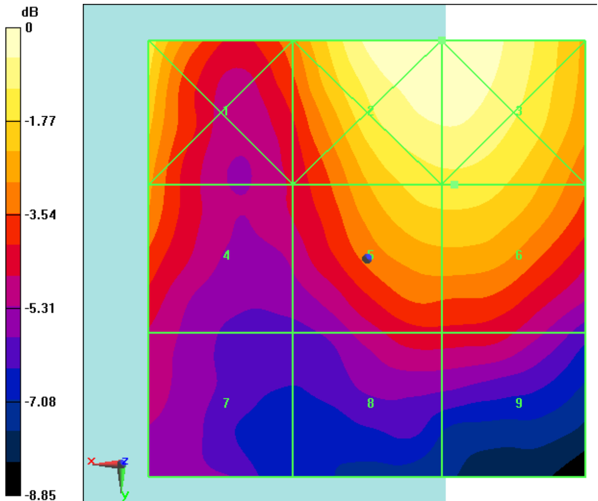
Fig B.40 HAC RF E-Field LTE Band41 Power Class 3 QPSK CH41490
