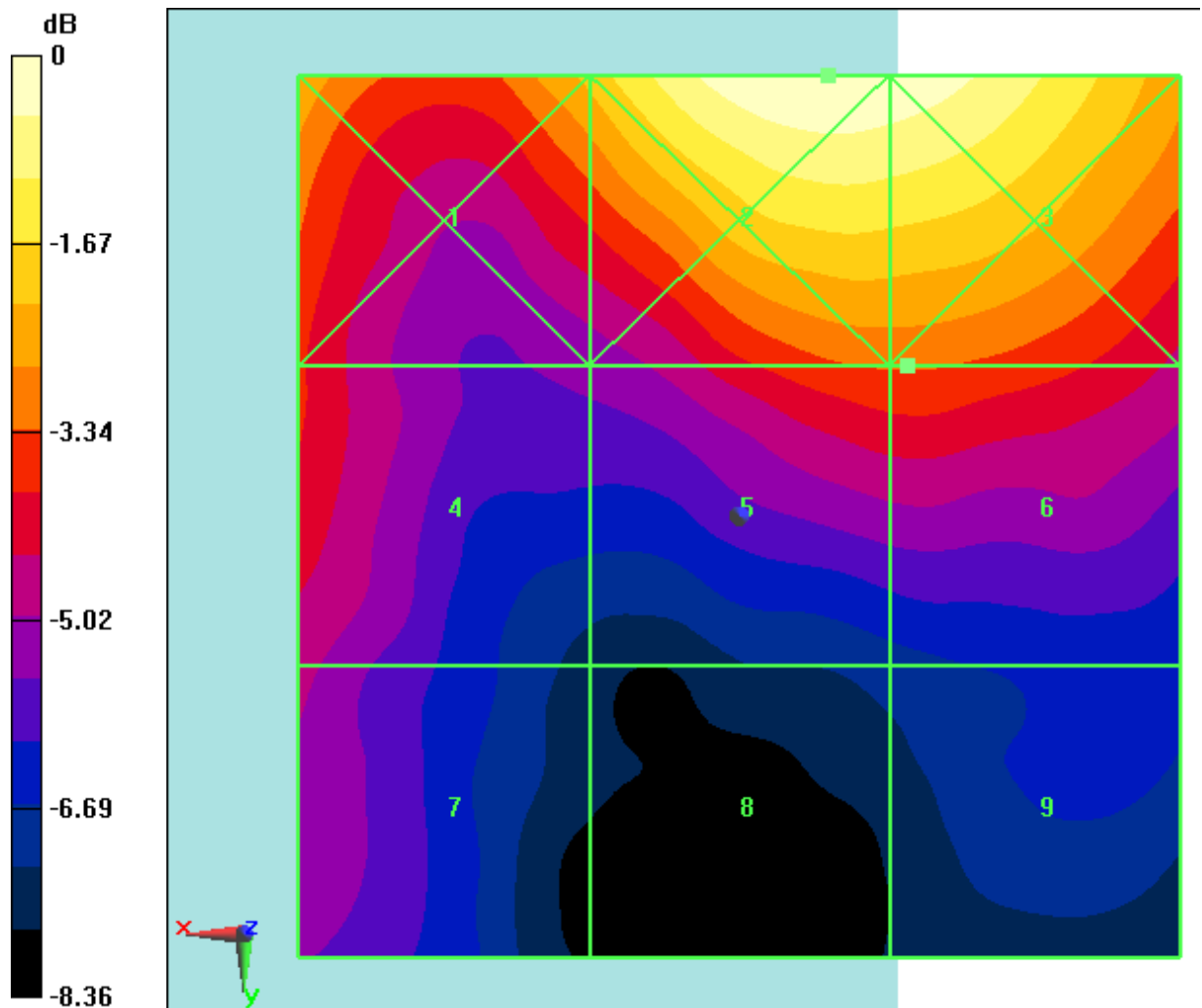
Fig B.34 HAC RF E-Field LTE Band41 Power Class 2 16QAM CH39750
