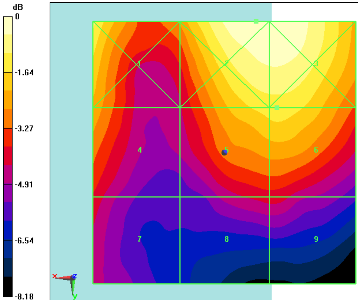
Fig B.35 HAC RF E-Field LTE Band41 Power Class 2 64QAM CH41490
