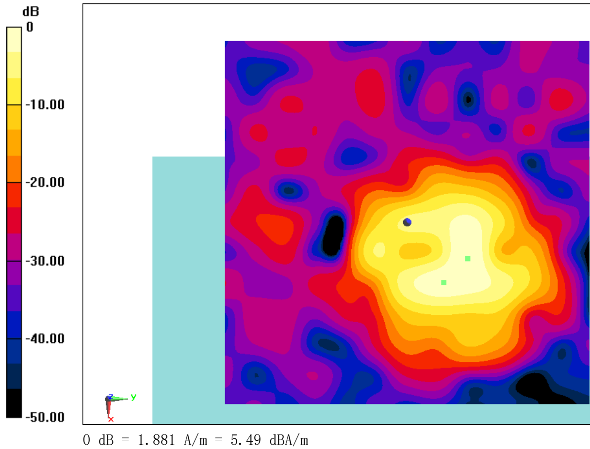
Fig B.42 T-Coil WiFi-5G
