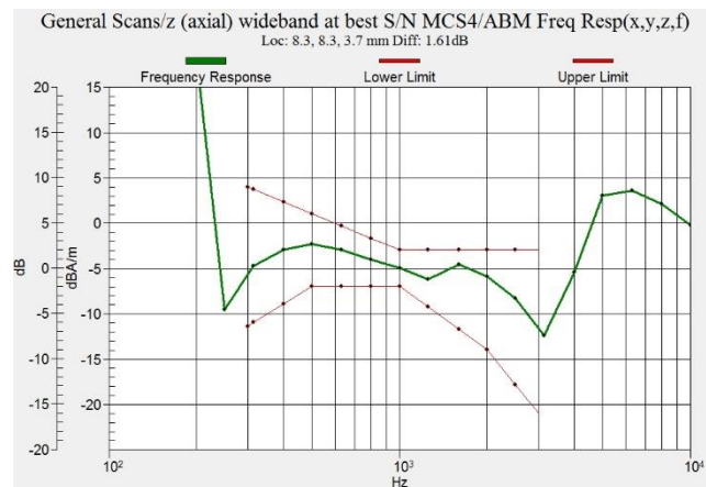
Figure C.20 Frequency Response of WiFi-2.4G
