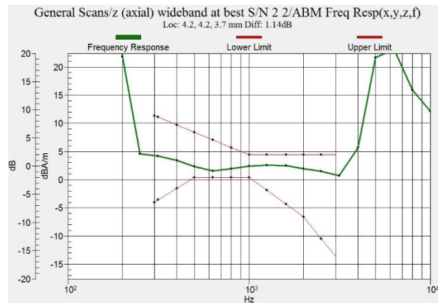
Figure C.22 Frequency Response of EDGE 1900 - OTT VoIP
