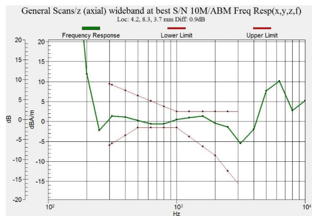
Figure C.12 Frequency Response of LTE B14
