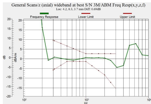
Figure C.24 Frequency Response of LTE B25 - OTT VoIP
