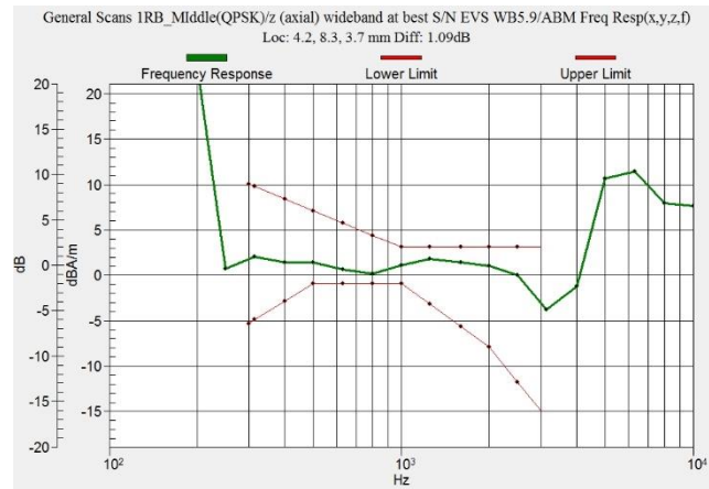
Figure C.25 Frequency Response of LTE B41 Power Class 2 - OTT VoIP
