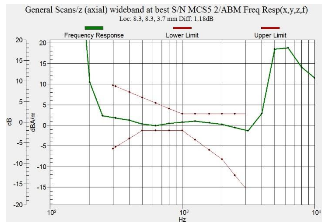
Figure C.27 Frequency Response of WiFi-5G - OTT VoIP
