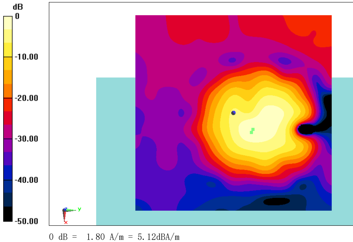
Fig B.50 T-Coil LTE B41
