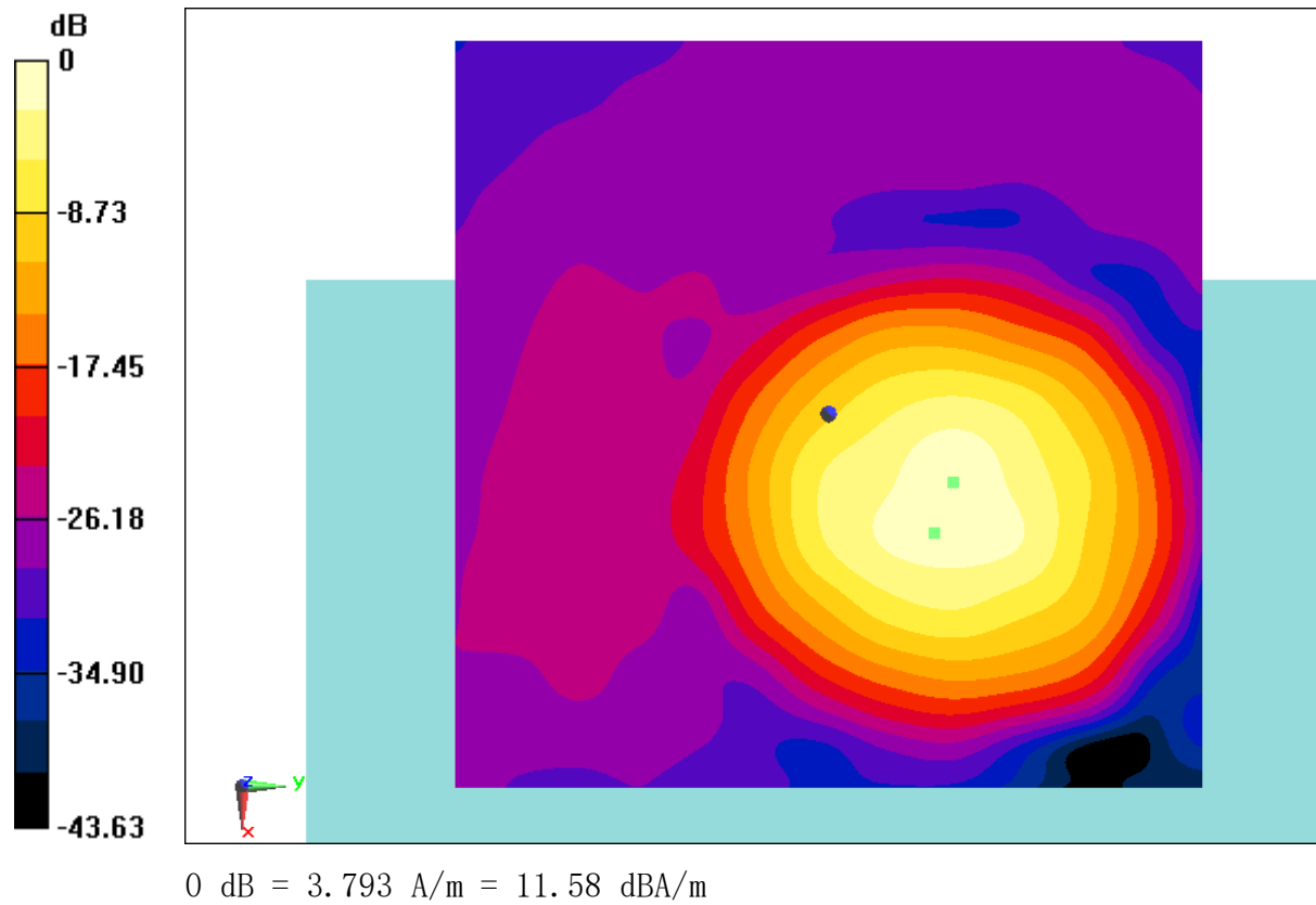
Fig B.54 T-Coil WiFi-5G
