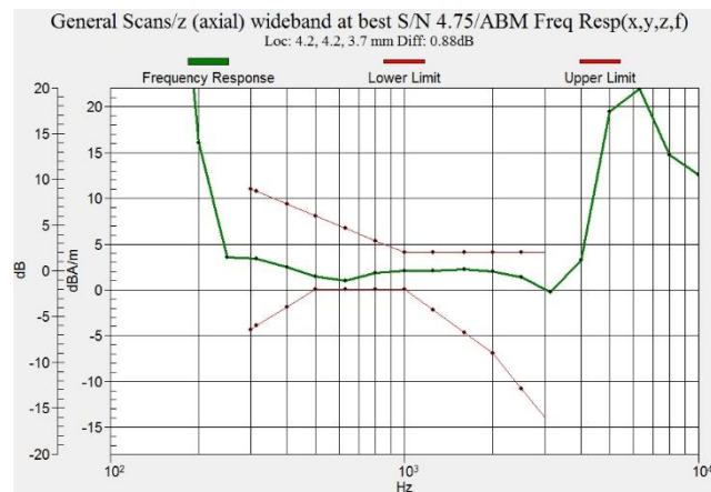
Figure C.23 Frequency Response of W850 - OTT VoIP
