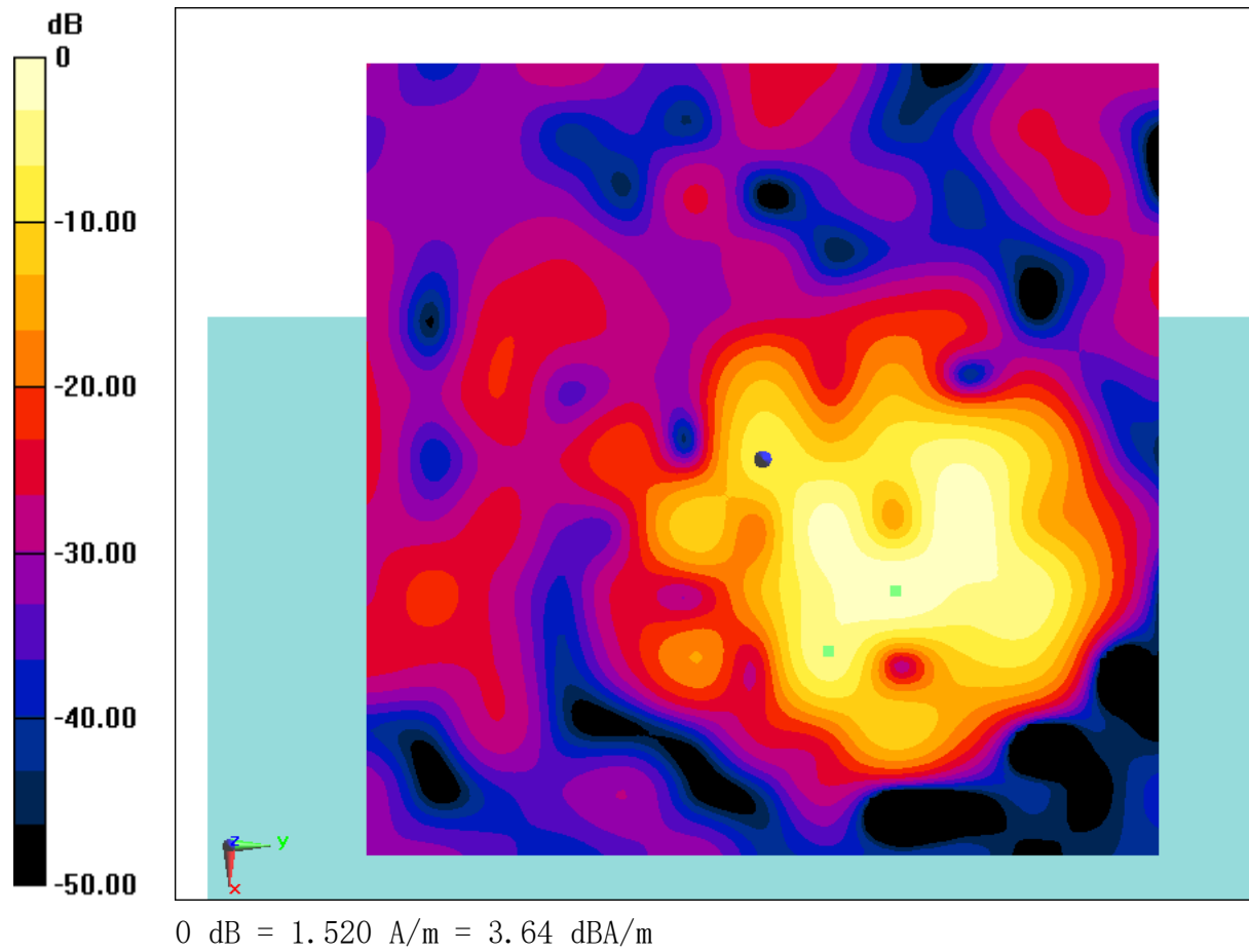
Fig B.40 T-Coil WiFi-2.4G
