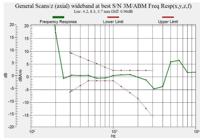
Figure C.14 Frequency Response of LTE B26
