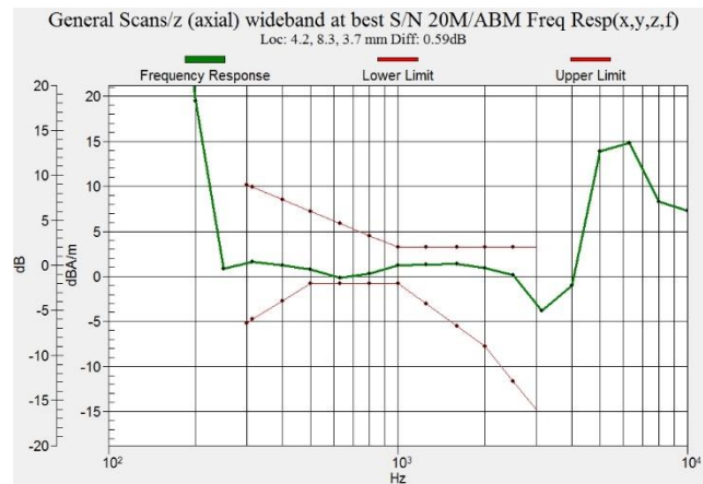
Figure C.19 Frequency Response of LTE B48
