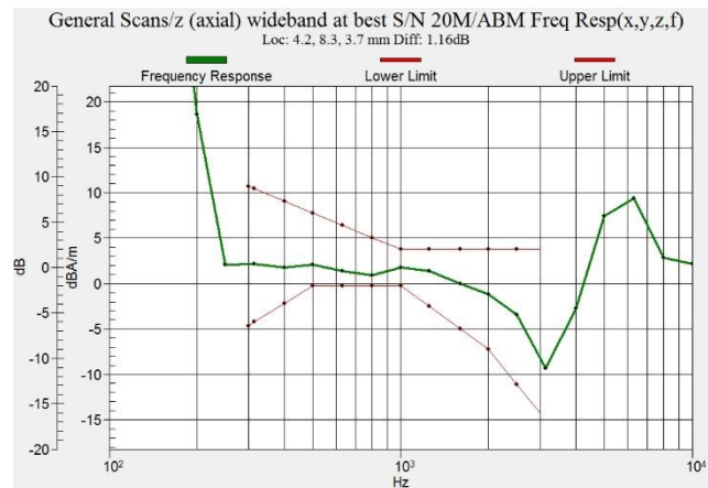
Figure C.16 Frequency Response of LTE B71
