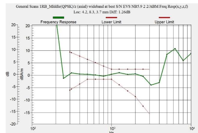
Figure C.18 Frequency Response of LTE B41 Power Class 3
