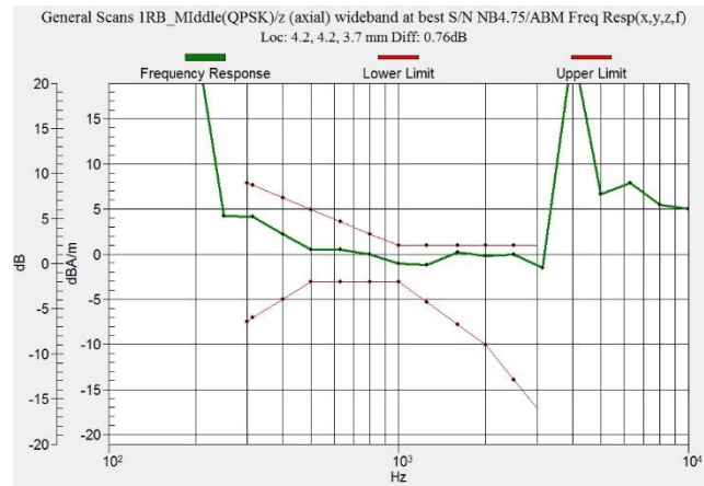
Figure C.13 Frequency Response of LTE B25
