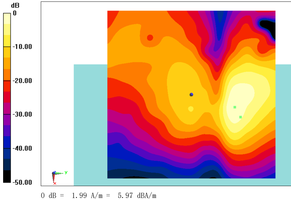
Fig B.49 T-Coil LTE B41
