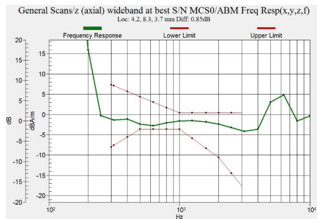
Figure C.21 Frequency Response of WiFi-5G
