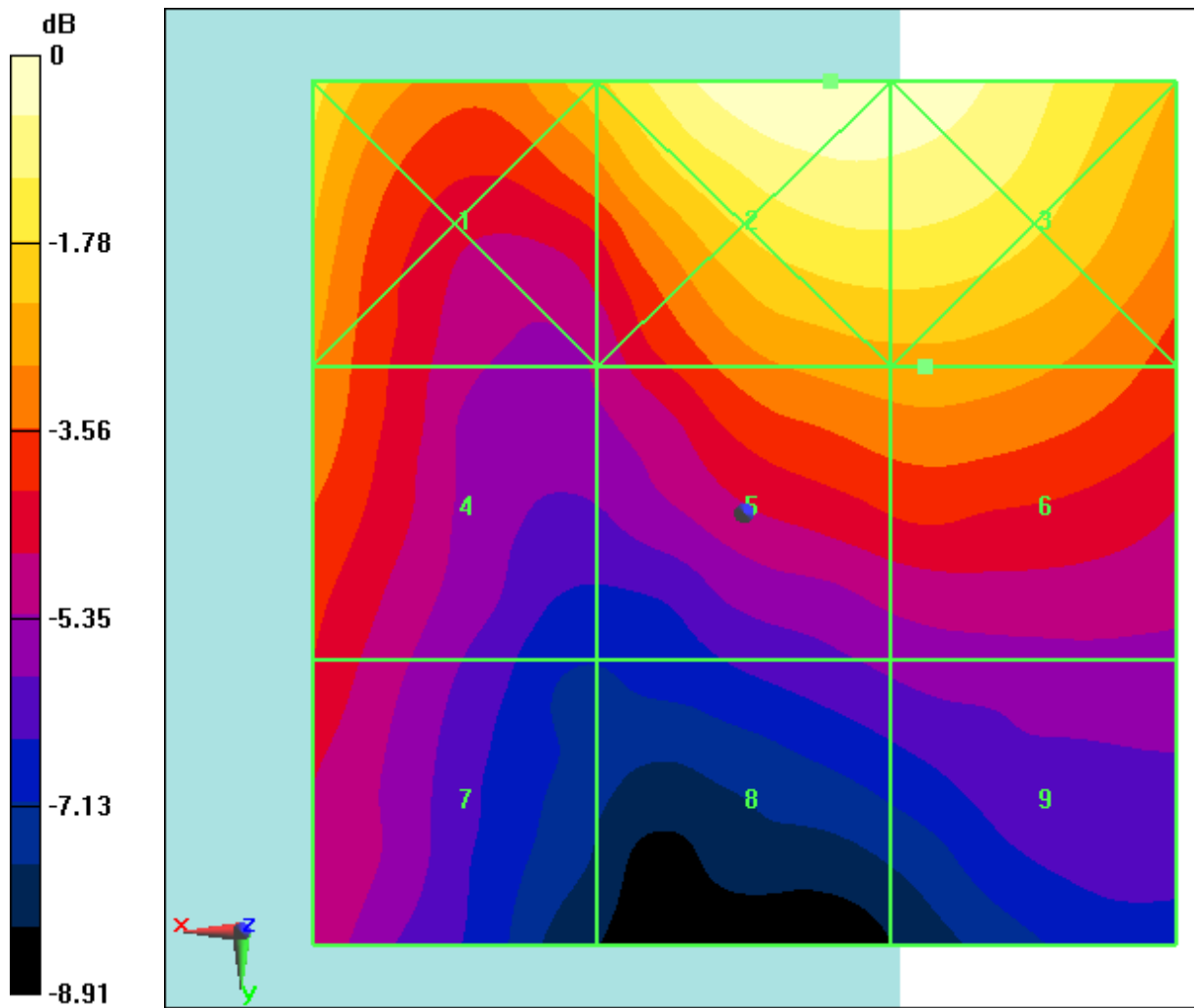
Fig B.27 HAC RF E-Field LTE Band41 Power Class 2 QPSK CH40620
