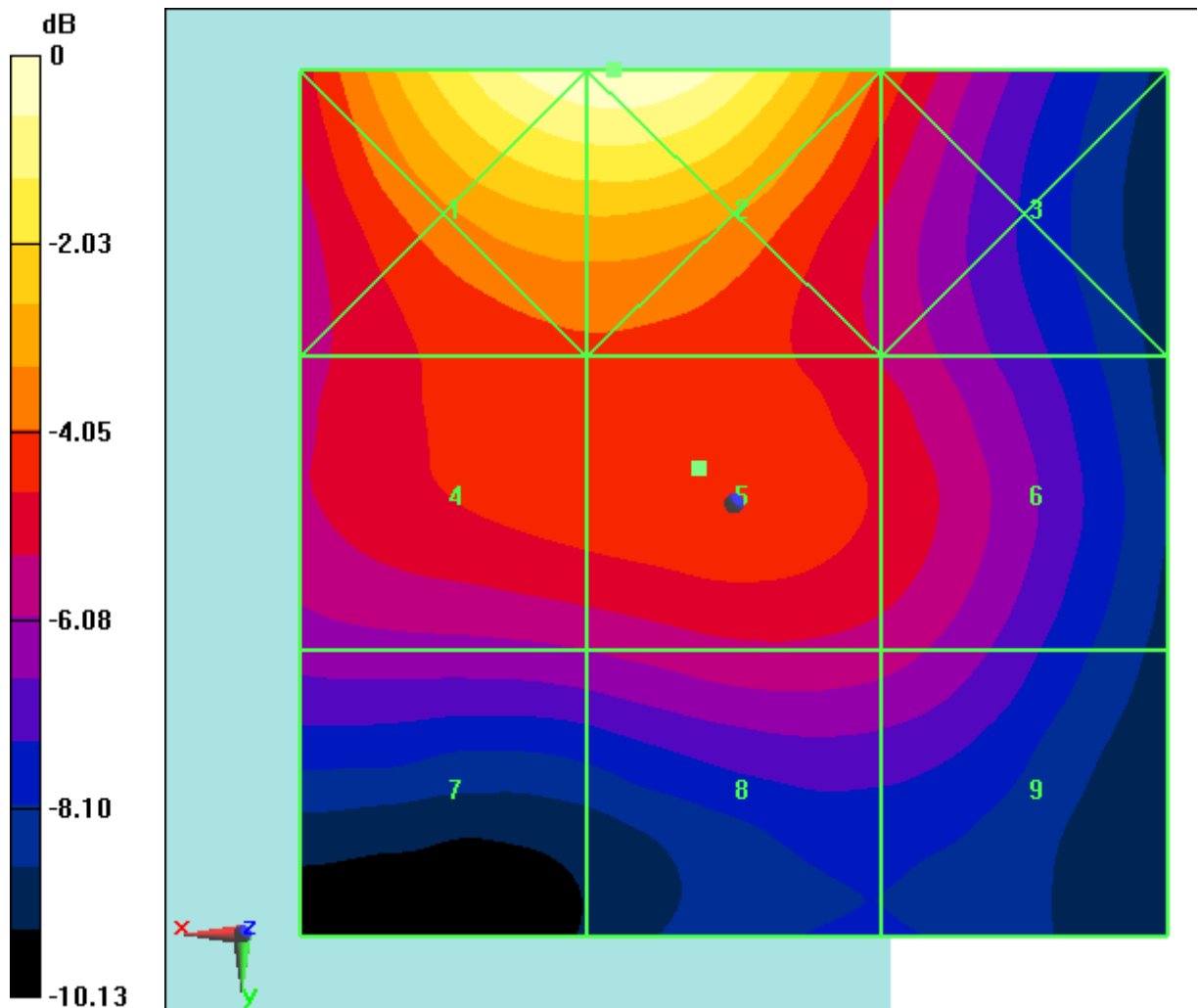
Fig B.19 HAC RF E-Field LTE Band48 16QAM CH56640
