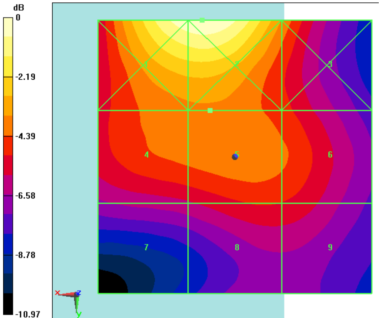
Fig B.21 HAC RF E-Field LTE Band48 16QAM CH55340
