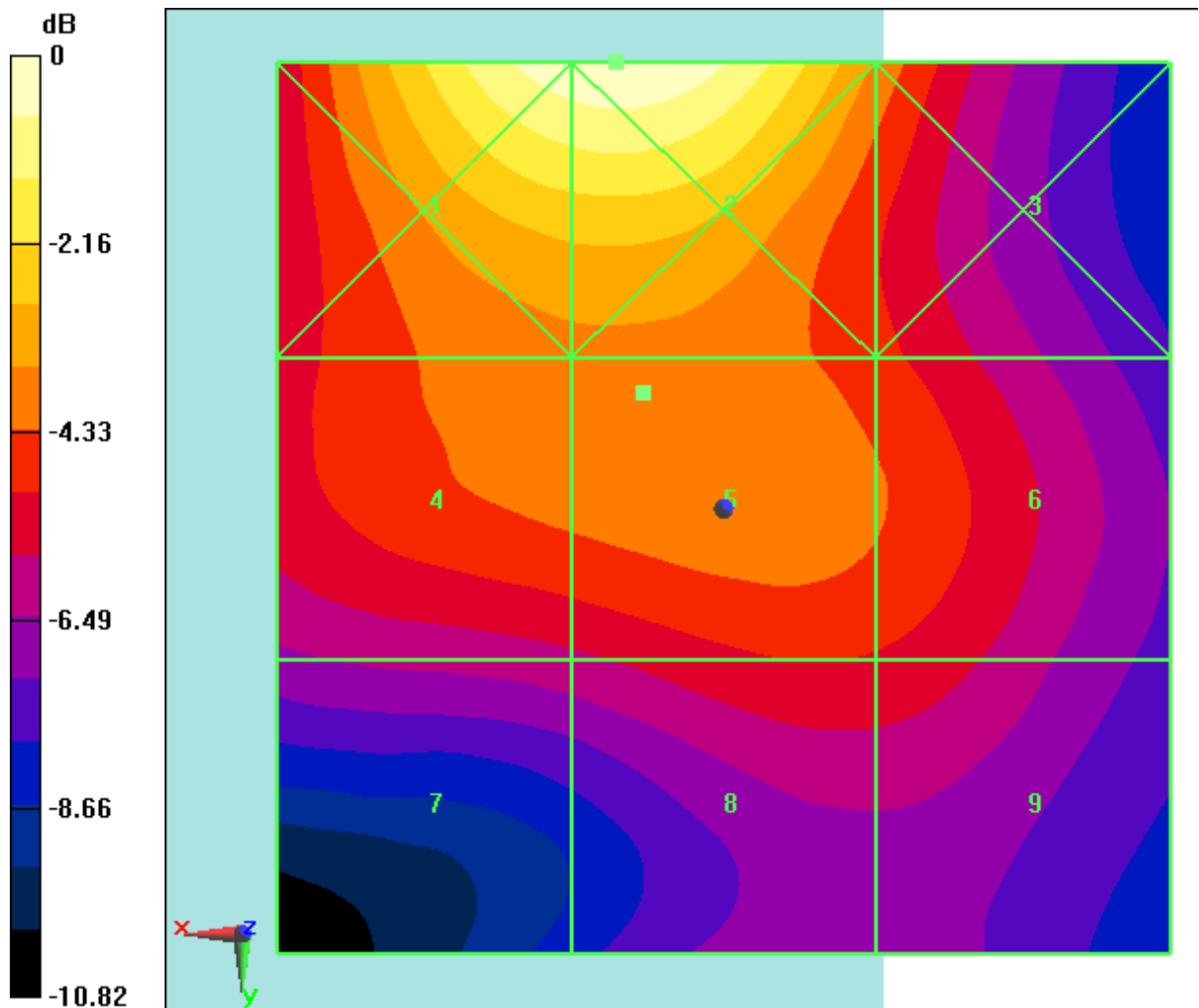
Fig B.24 HAC RF E-Field LTE Band48 64QAM CH55340
