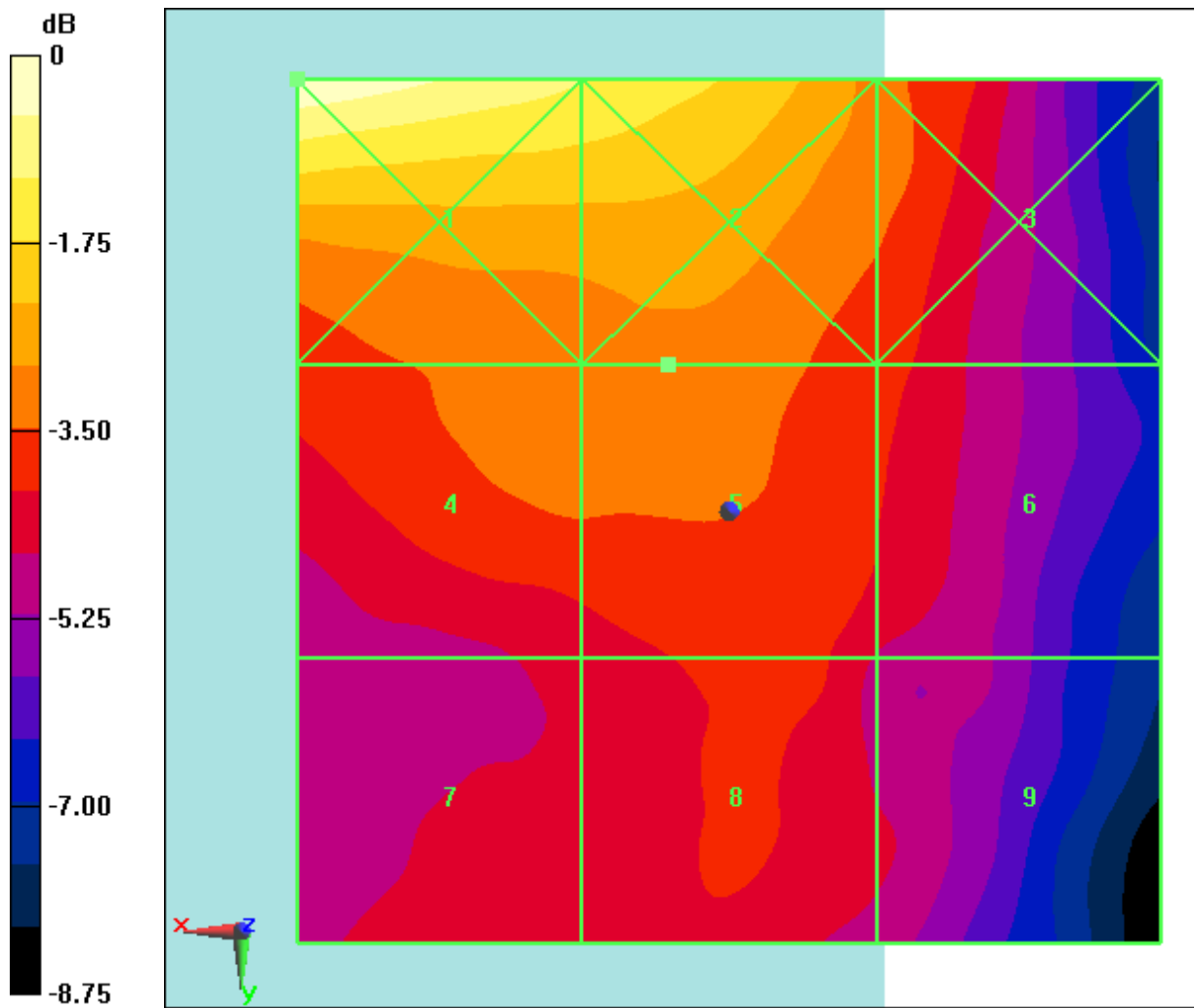
Fig B.7 HAC RF E-Field CDMA BC0 High
