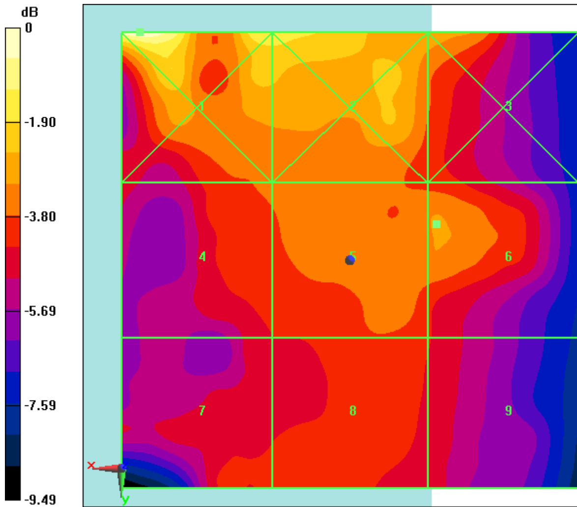
Fig B.1 HAC RF E-Field GSM 850 High
