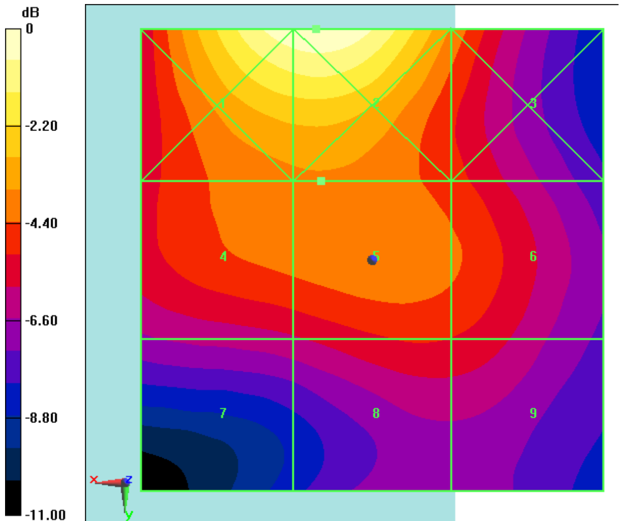
Fig B.18 HAC RF E-Field LTE Band48 QPSK CH55340
