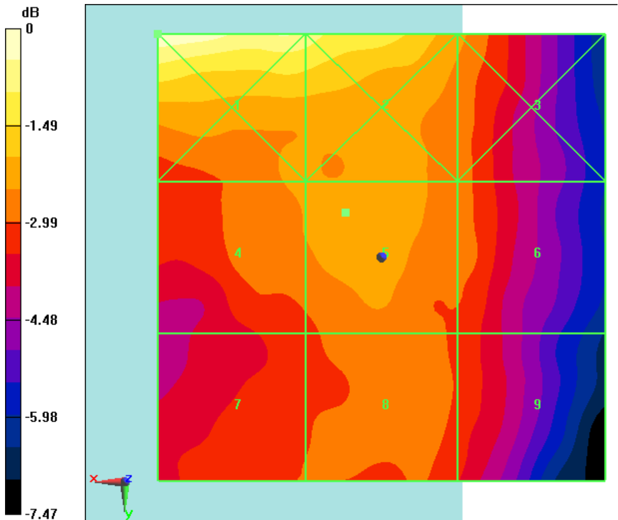
Fig B.8 HAC RF E-Field CDMA BC0 Middle
