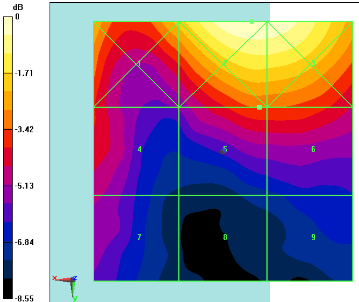
Fig B.44 HAC RF E-Field LTE Band41 Power Class 3 QPSK CH39750
