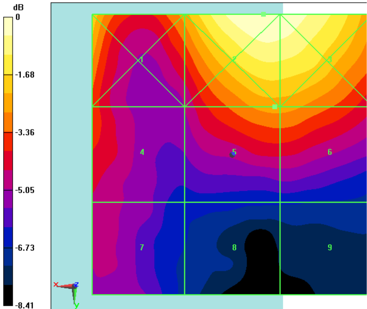
Fig B.46 HAC RF E-Field LTE Band41 Power Class 3 16QAM CH41055
