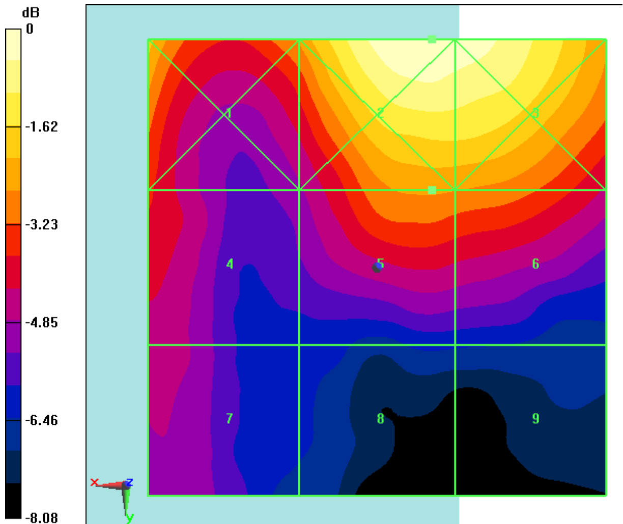
Fig B.51 HAC RF E-Field LTE Band41 Power Class 3 64QAM CH41055
