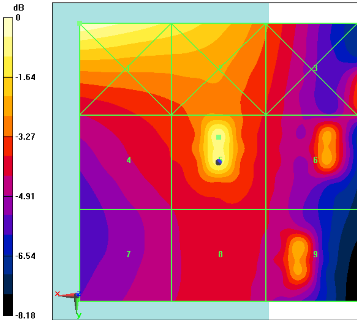
Fig B.3 HAC RF E-Field GSM 850 Low
