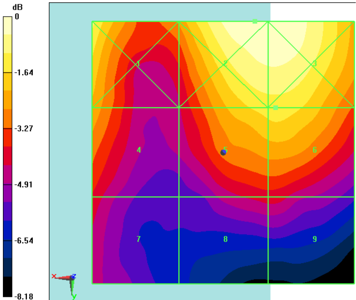
Fig B.50 HAC RF E-Field LTE Band41 Power Class 3 64QAM CH41490
