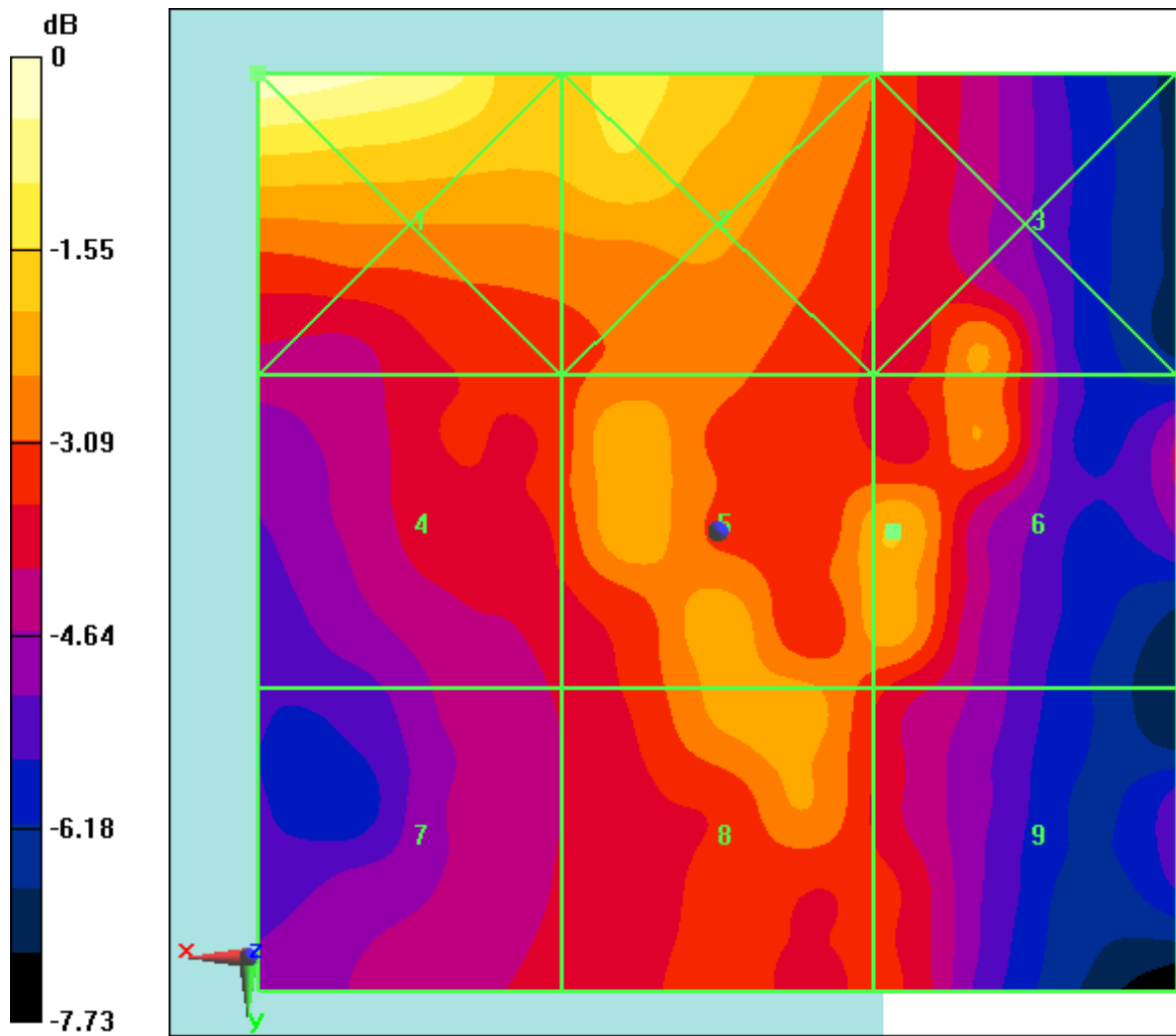
Fig B.2 HAC RF E-Field GSM 850 Middle
