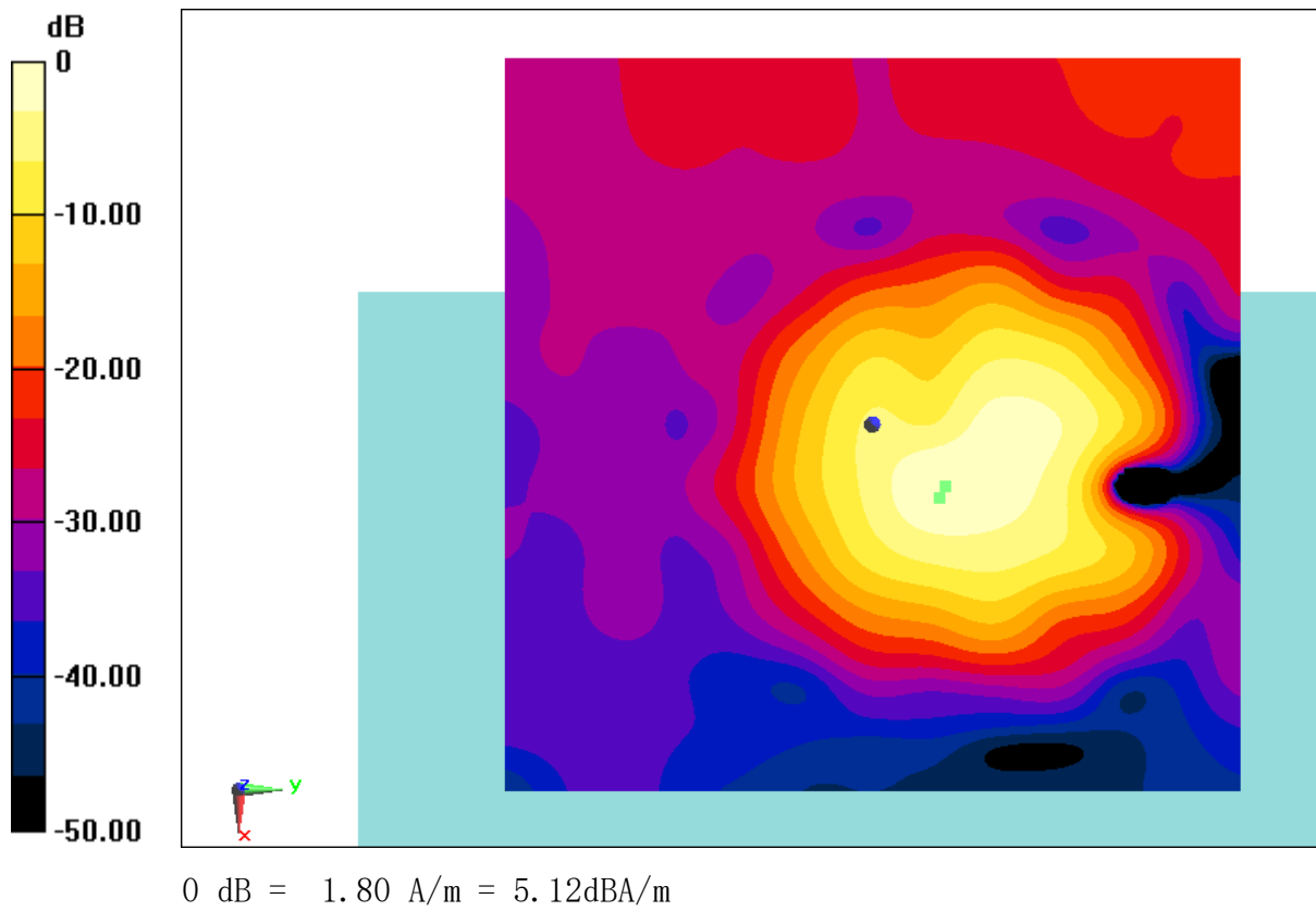
Fig B.46 T-Coil LTE B41
