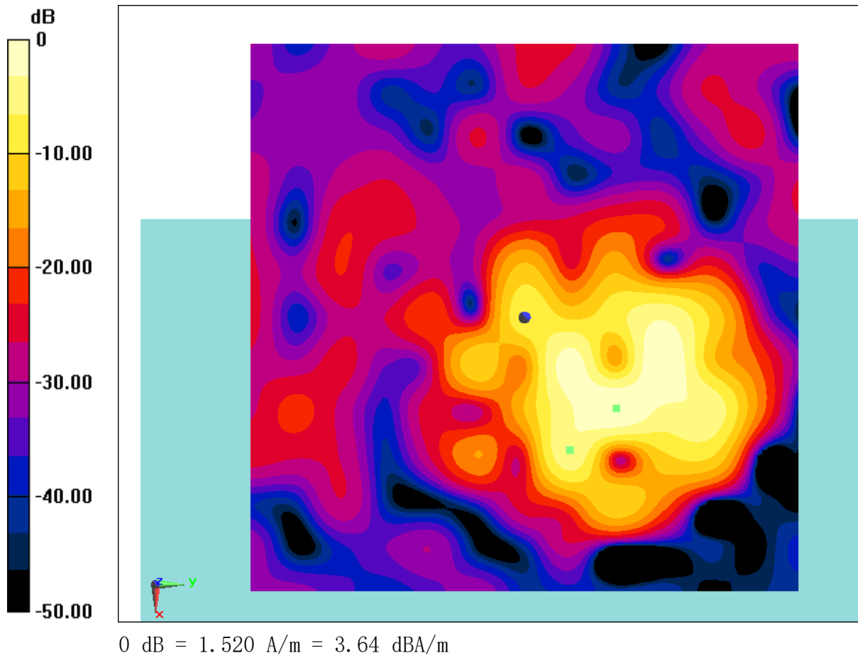
Fig B.36 T-Coil WiFi-2.4G
