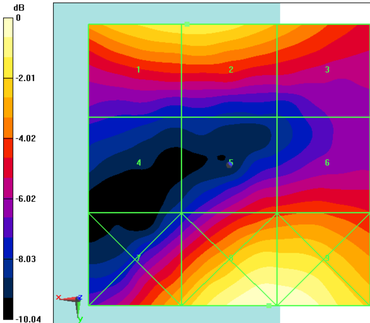
Fig B.5 HAC RF E-Field GSM 1900 Middle
