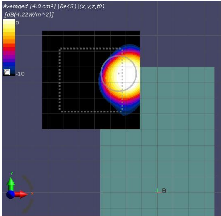
Figure 8-2: 4cm2-averaged power density distribution measured at input.power.limit of 3.3 dBm on the back surface for n261 beam 20
