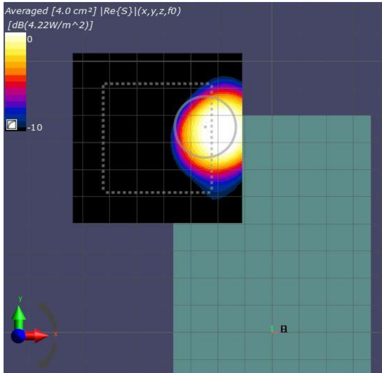
Figure 8-2: 4cm2-averaged power density distribution measured at input.power.limit of 3.3 dBm on the back surface for n261 beam 20
