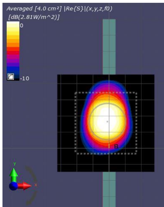
Figure 8-3: 4cm2-averaged power density distribution measured at input.power.limit of 2.1 dBm on the Right Side for n260 beam 31
