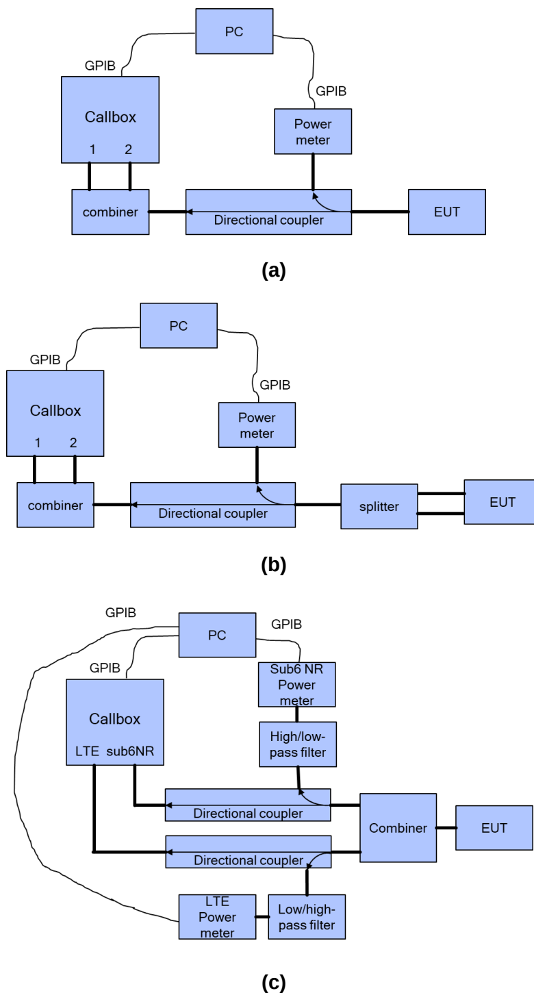
Figure 6-1Conducted power measurement setup
