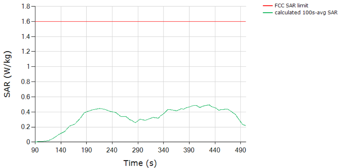
SAR (Test Sequence 2) Tech: LTE, Band 71
