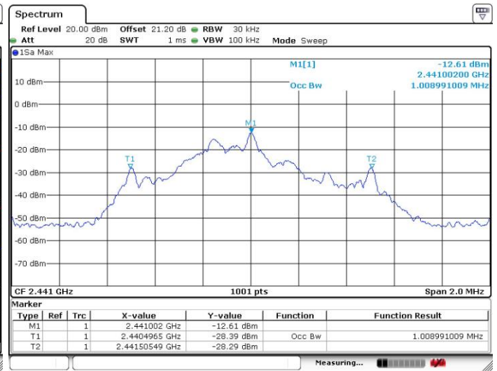
99% Bandwidth Plot on 2441MHz
