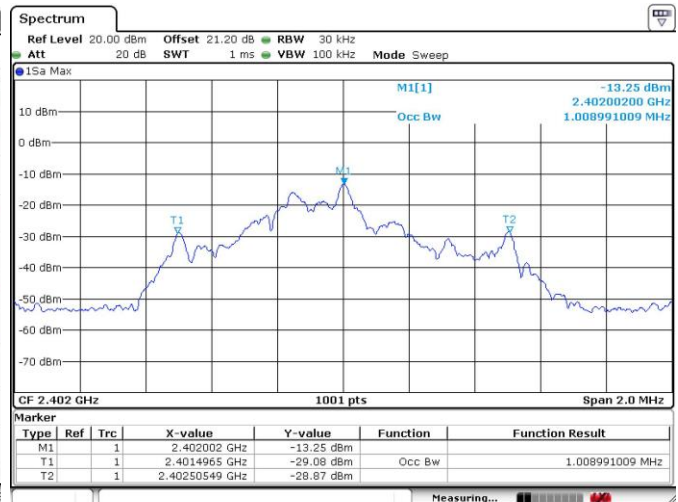
99% Bandwidth Plot on 2402MHz
