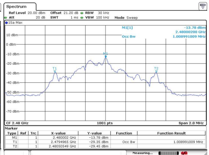
99% Bandwidth Plot on 2480MHz
