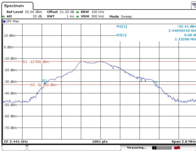
20 dB Bandwidth Plot on 2441MHz
