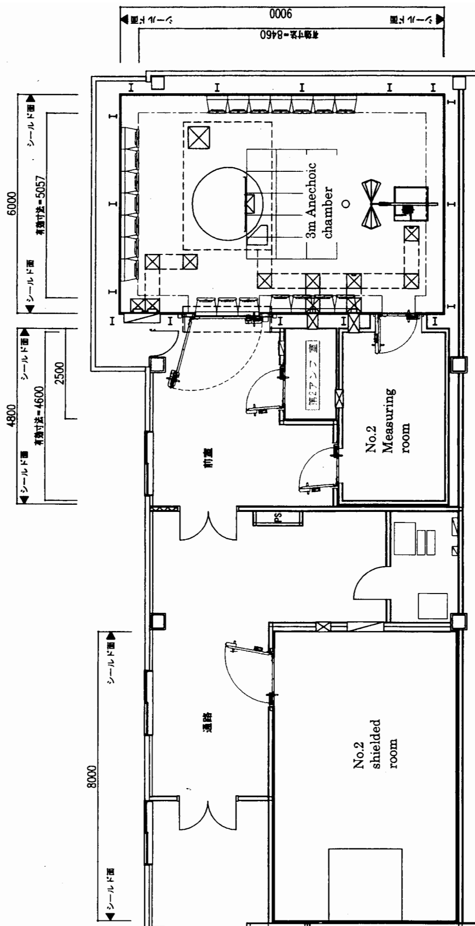
Fig.2-2. Physical Layout of the Semi-anechoic Chamber (Top View)
