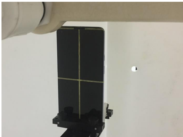
Top Side, Test Separation 9 mm
