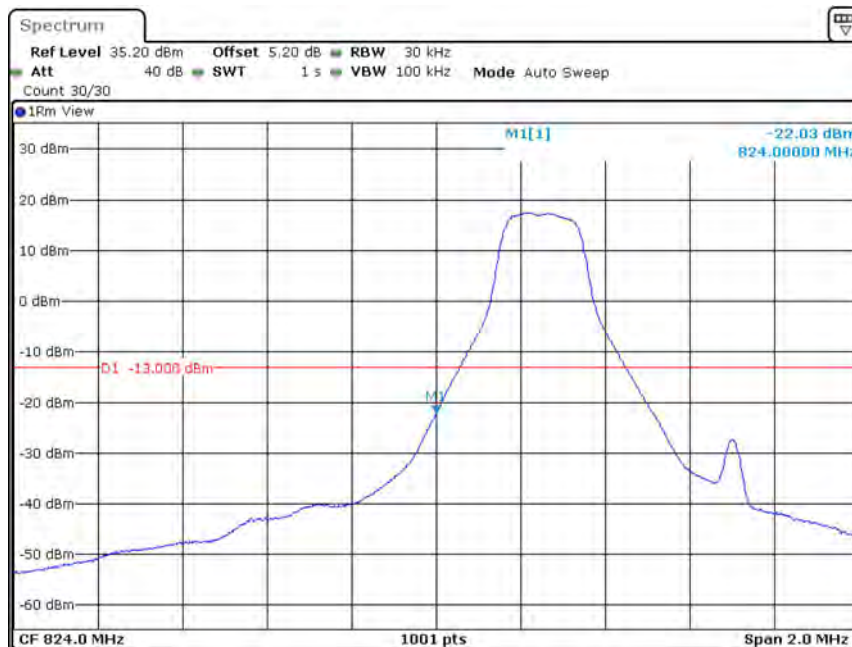
Band26-1.4MHz-QPSK-26797-1RB#0
