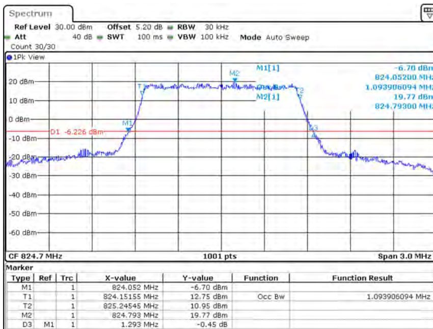
Band26-1.4MHz-QPSK-26797-6RB#0-1.094
