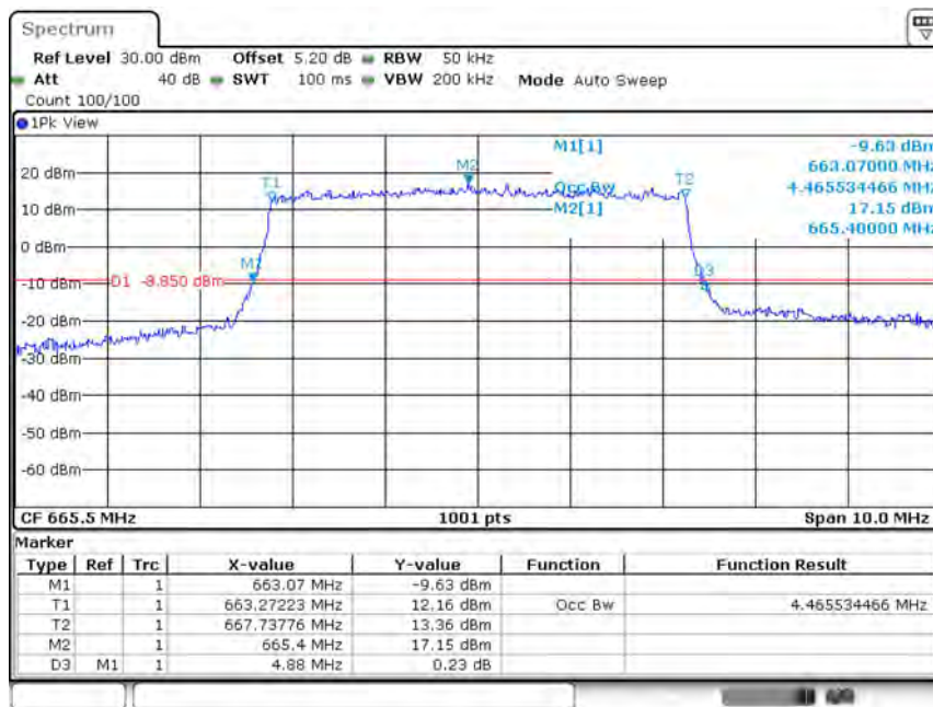
Band71-5MHz-QPSK-133147-25RB#0-4.466
