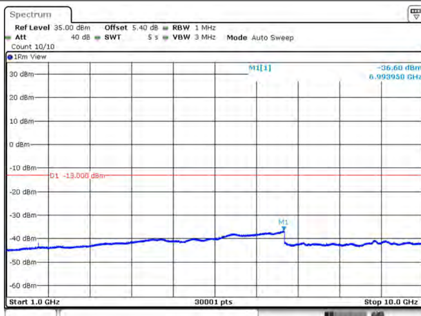
Band5-10MHz-16QAM-20600-1RB#0-Range2:1000~10000MHz
