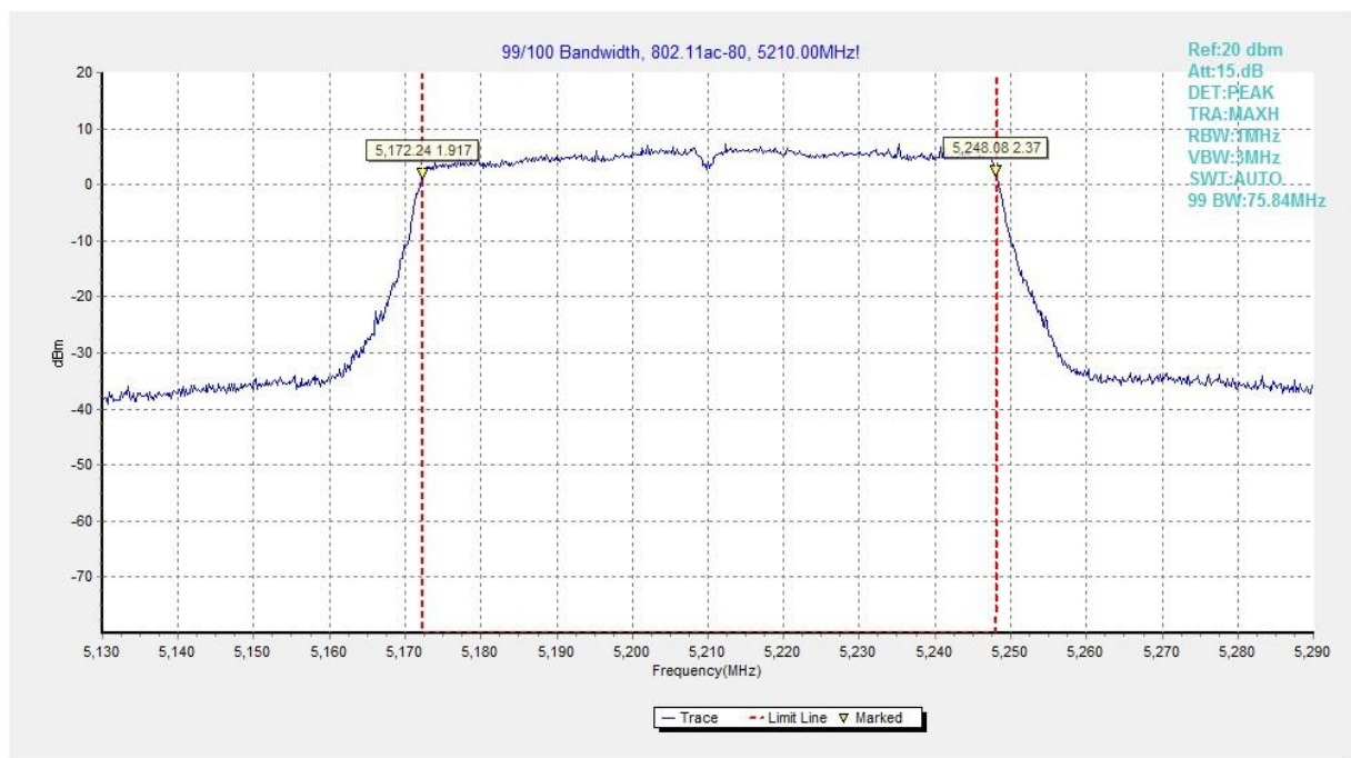
Fig.92 99% Occupied bandwidth (802.11ac-HT80, 5210MHz)
