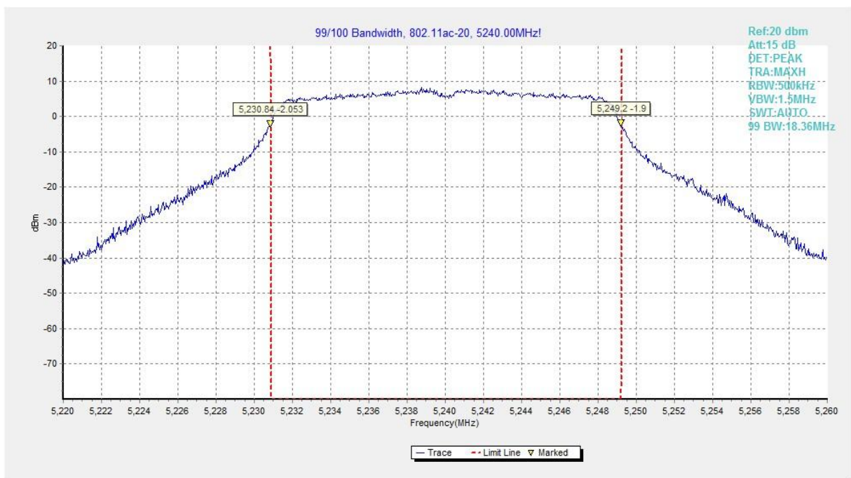
Fig.87 99% Occupied bandwidth (802.11ac-HT20, 5240MHz)
