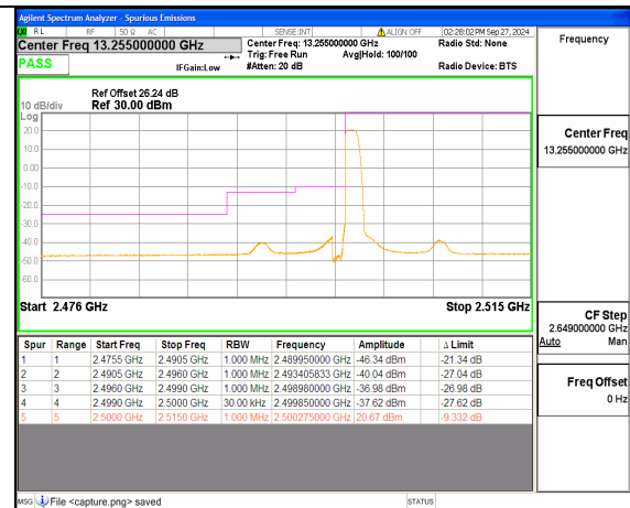
n7 15M DFT-s-OFDM BPSK Edge 1RB Left Low
