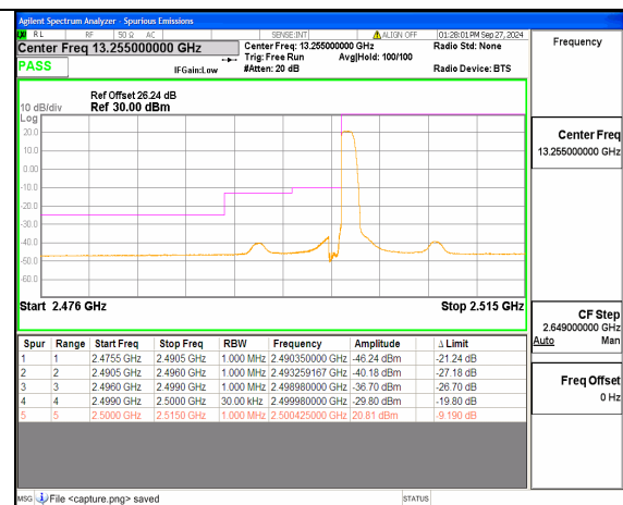
n7 15M DFT-s-OFDM QPSK Edge 1RB Left Low
