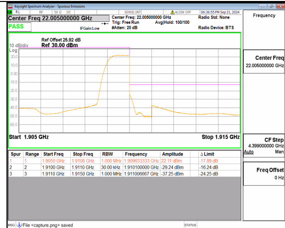
n2 5M DFT-s-OFDM QPSK Edge_1RB_Right High
