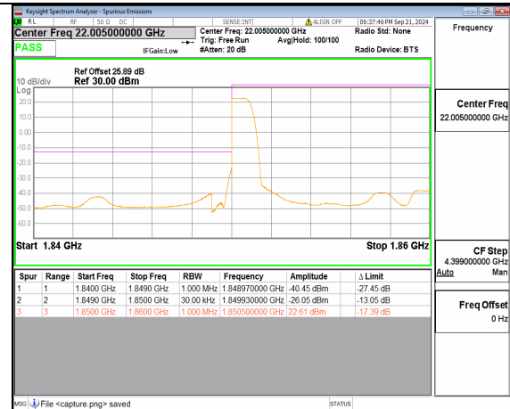
n2 10M DFT-s-OFDM BPSK Edge_1RB_Left Low
