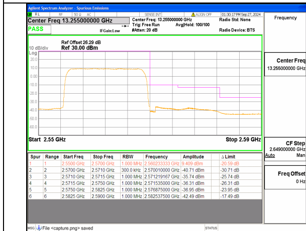
n7 15M DFT-s-OFDM QPSK Outer_Full High
