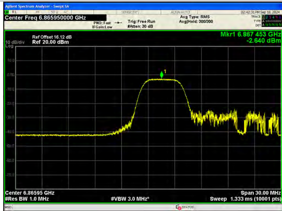
PSD NVNT ax20 52@37 6875MHz Ant13 MIMO
