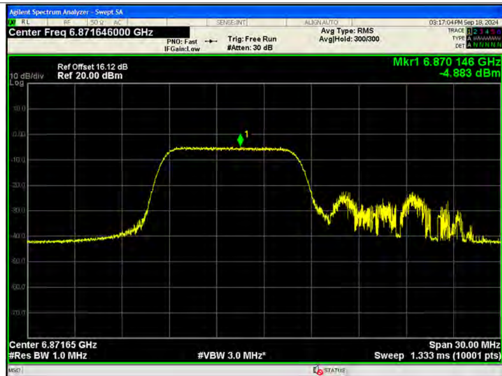
PSD NVNT ax20 106@53 6875MHz Ant12 SISO
