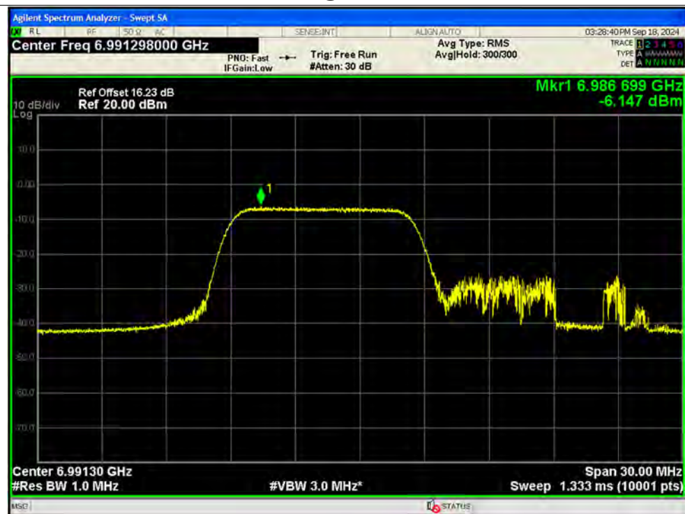
PSD NVNT ax20 106@53 6995MHz Ant13 MIMO
