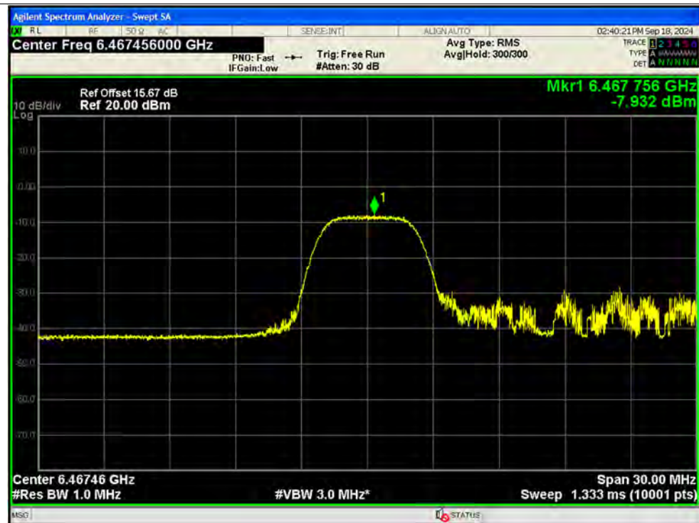
PSD NVNT ax20 52@37 6475MHz Ant13 MIMO
