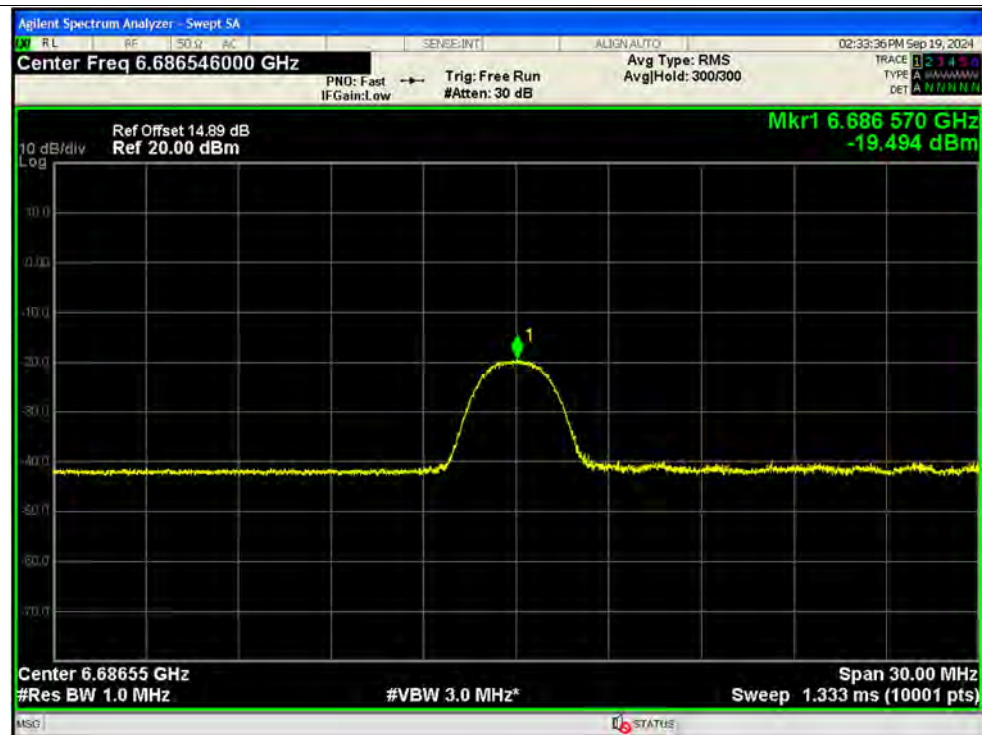
PSD NVNT ax20 26@0 6695MHz Ant13 MIMO
