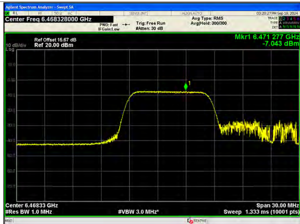
PSD NVNT ax20 106@53 6475MHz Ant13 SISO
