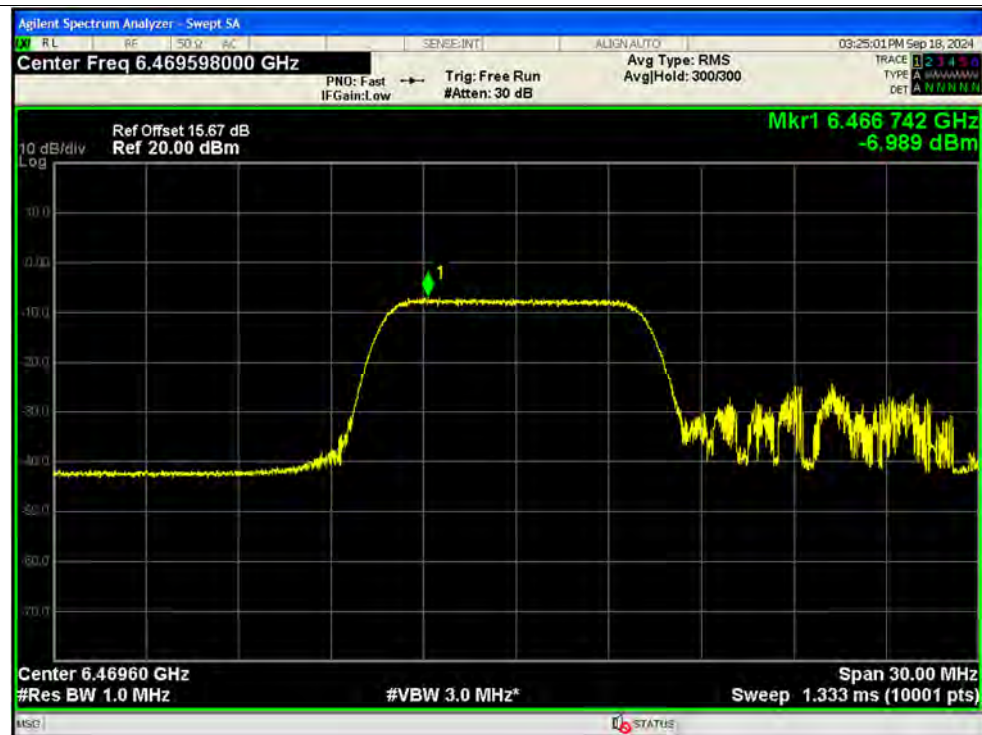
PSD NVNT ax20 106@53 6475MHz Ant13 MIMO
