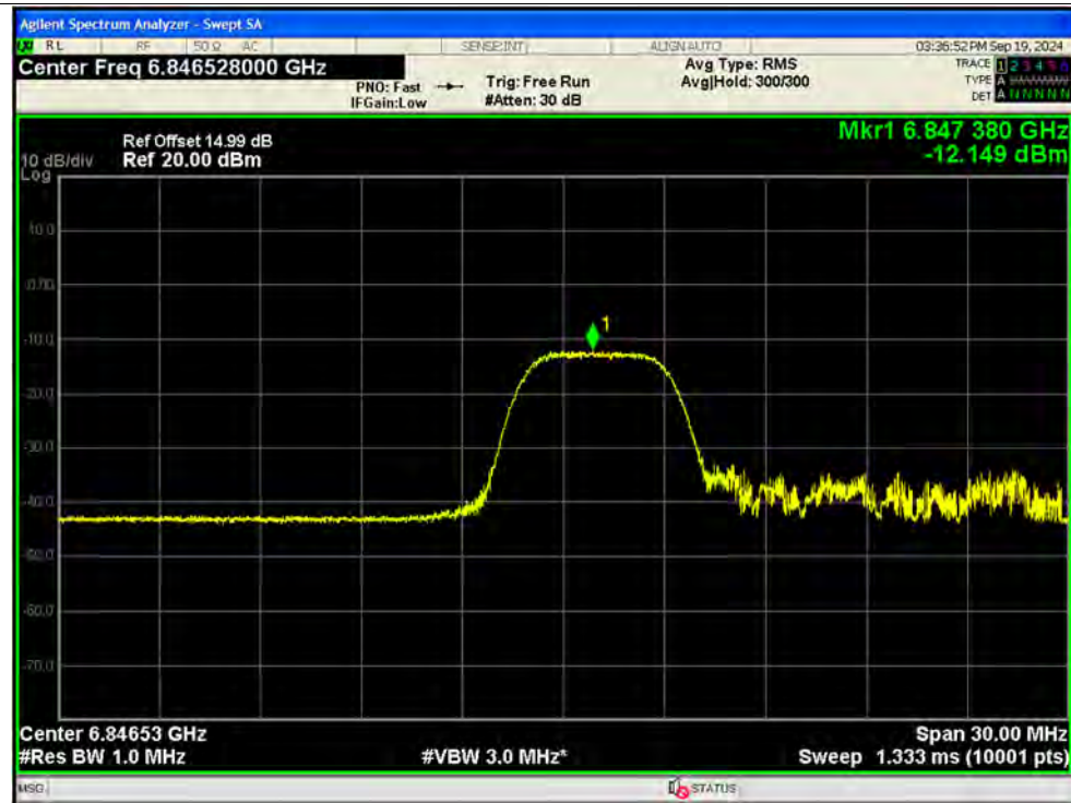
PSD NVNT ax20 52@37 6855MHz Ant13 MIMO
