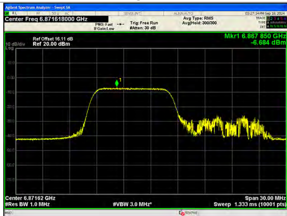
PSD NVNT ax20 106@53 6875MHz Ant13 MIMO
