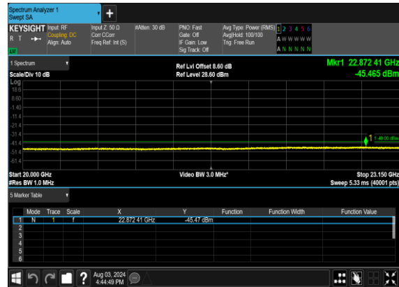
N30(10M)_DFT-s- OFDM_BPSK_Edge_1RB_Left_Low_CH
