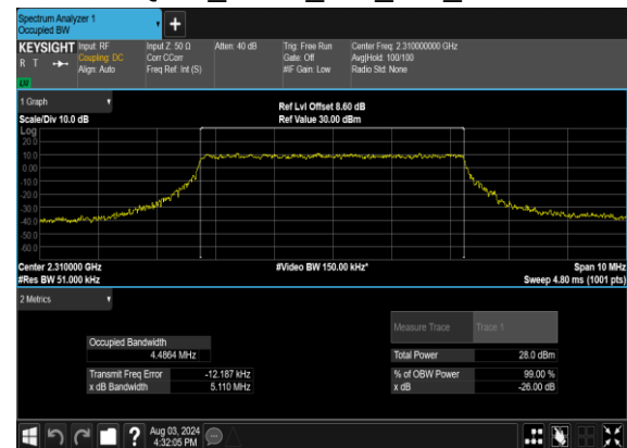
N30(5M)_CP-OFDM_16 QAM_Outer_Full_Mid_CH
