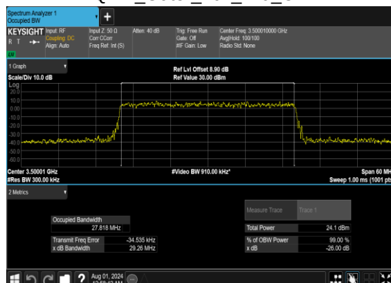
N77(30M)_CP-OFDM_256 QAM_Outer_Full_Mid_CH
