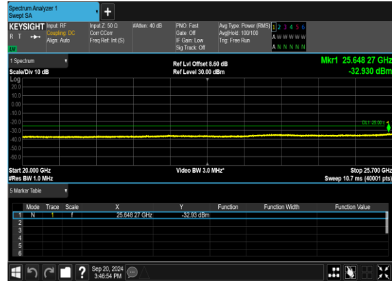
N7(50M)_DFT-s- OFDM_QPSK_Edge_1RB_Left_Mid_CH
