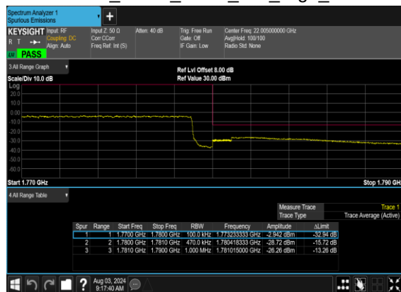
N66(45M)_DFT-s- OFDM_BPSK_Outer_Full_High_CH
