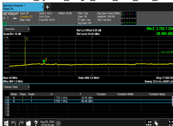
N66(25M)_DFT-s- OFDM_QPSK_Edge_1RB_Left_Mid_CH
