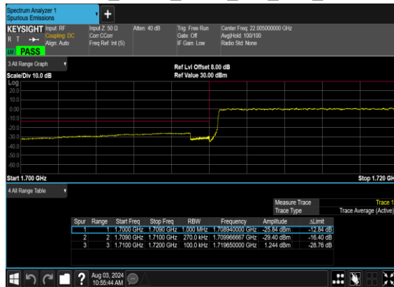
N66(25M)_DFT-s- OFDM_QPSK_Outer_Full_Low_CH
