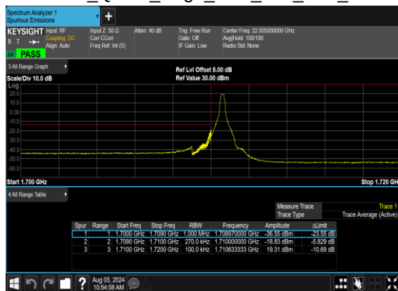
N66(25M)_DFT-s- OFDM_QPSK_Edge_1RB_Left_Low_CH
