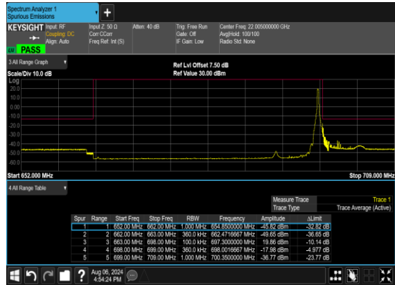
N71(35M)_DFT-s- OFDM_QPSK_Edge_1RB_Right_High_CH
