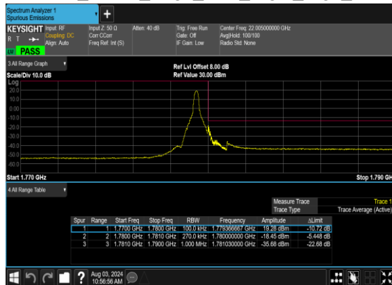
N66(25M)_DFT-s- OFDM_QPSK_Edge_1RB_Right_High_CH
