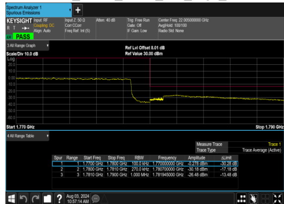
N66(25M)_DFT-s- OFDM_BPSK_Outer_Full_High_CH
