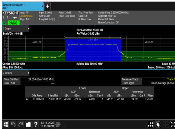
N48(10M)_DFT-s-OFDM_PI_2- BPSK_Outer_Full_Low_CH
