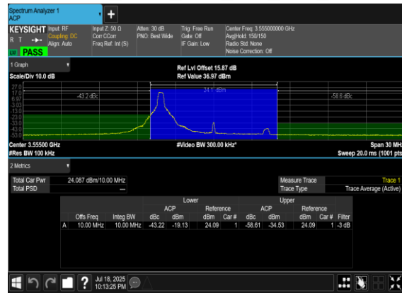
N48(10M)_DFT-s-OFDM_PI_2- BPSK_Edge_1RB_Left_Low_CH
