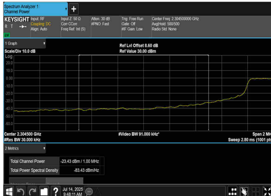
N30(10M)_DFT-s- OFDM_BPSK_Outer_Full_Low_CH_CHP_PASS
