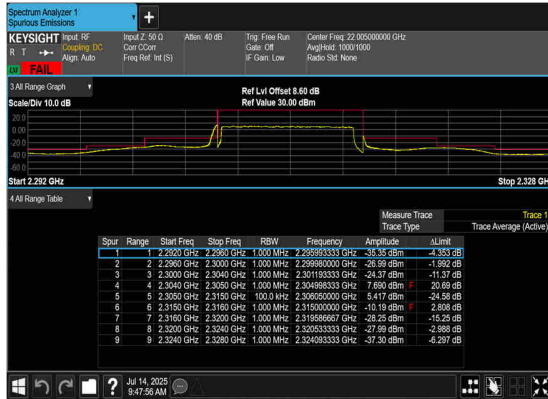
N30(10M)_DFT-s- OFDM_BPSK_Outer_Full_Low_CH
