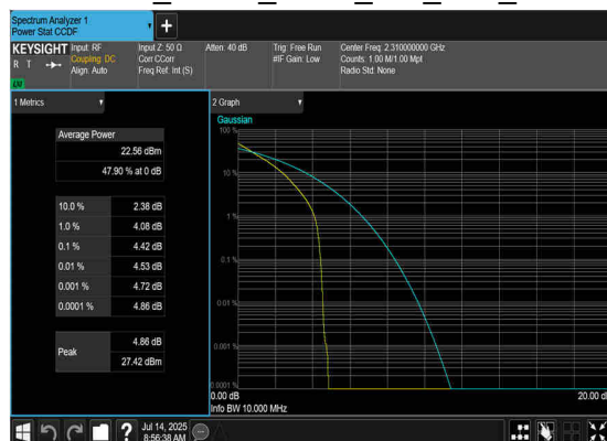
N30(10M)_DFT-s-OFDM_QPSK_Outer_Full_Low_CH
