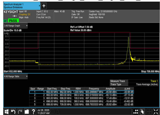
N71(35M)_DFT-s- OFDM_QPSK_Edge_1RB_Right_Mid_CH
