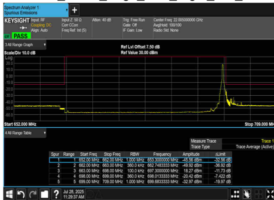
N71(35M)_DFT-s- OFDM_BPSK_Edge_1RB_Right_Mid_CH
