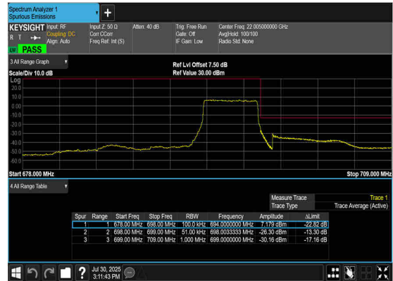
N71(5M)_DFT-s- OFDM_QPSK_Outer_Full_High_CH
