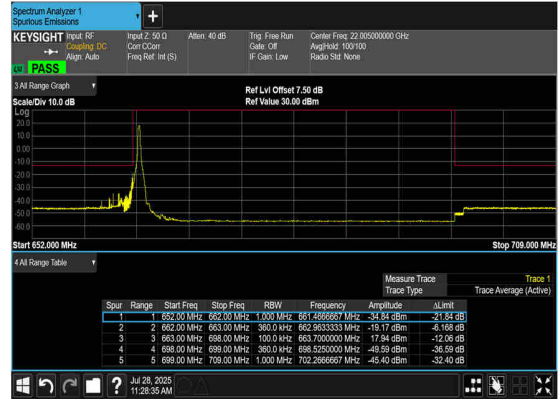
N71(35M)_DFT-s- OFDM_QPSK_Edge_1RB_Left_Mid_CH
