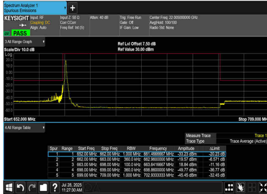
N71(35M)_DFT-s- OFDM_BPSK_Edge_1RB_Left_Mid_CH
